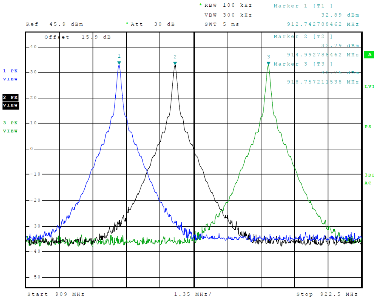
Figure 3 Transmitter Output Across Frequency Band EPC
