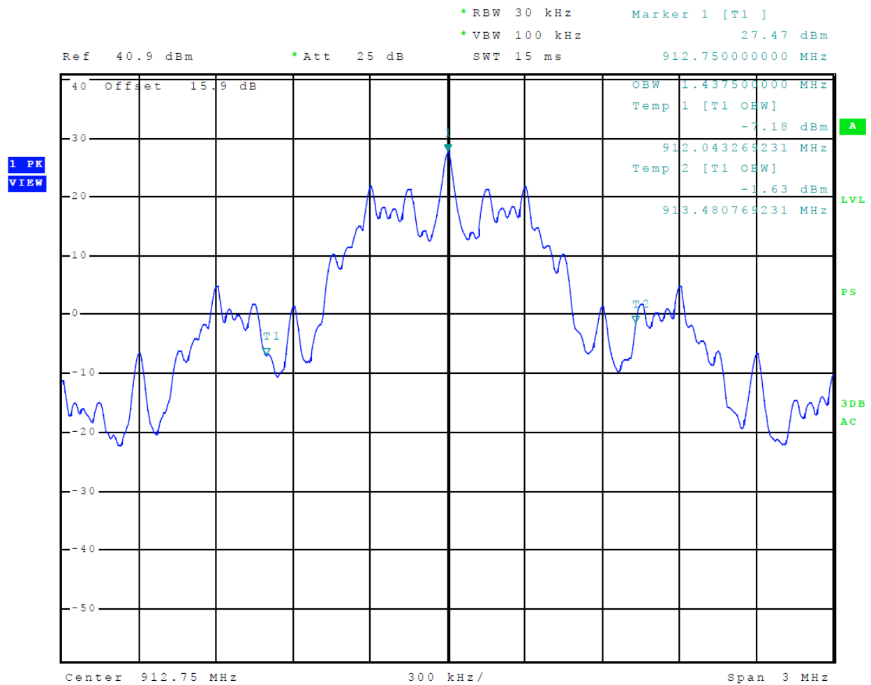
Figure 12 Occupied Bandwidth Title 21
