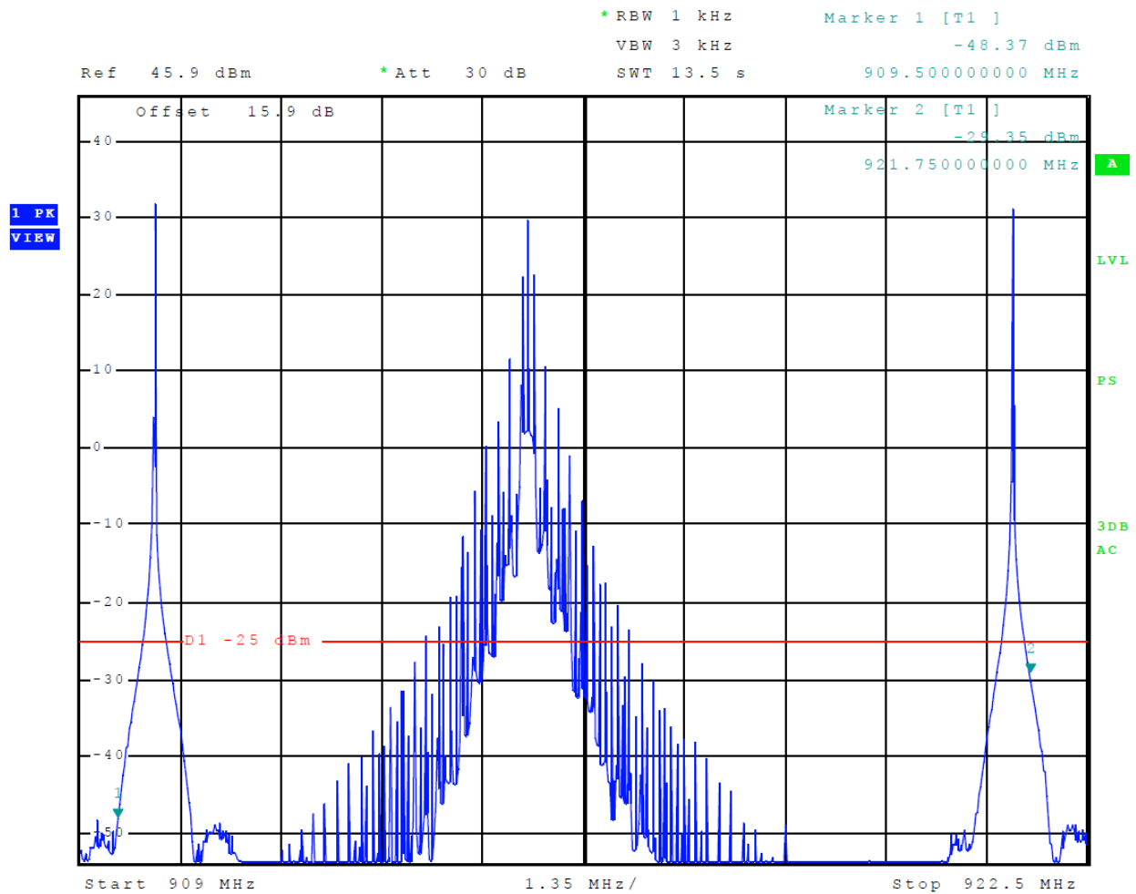
Figure 17 Emissions Mask SeGo
