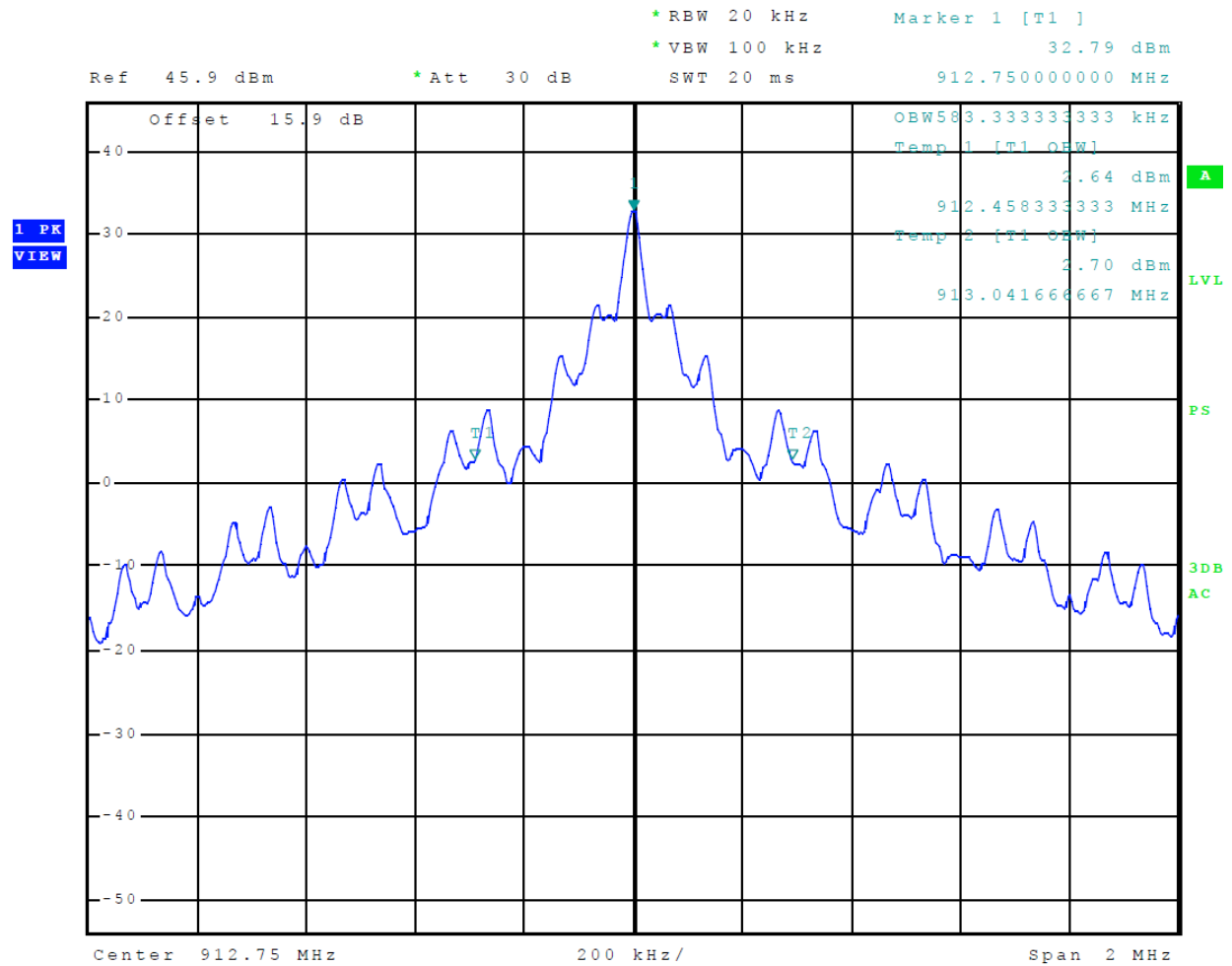
Figure 9 Occupied Bandwidth EPC
