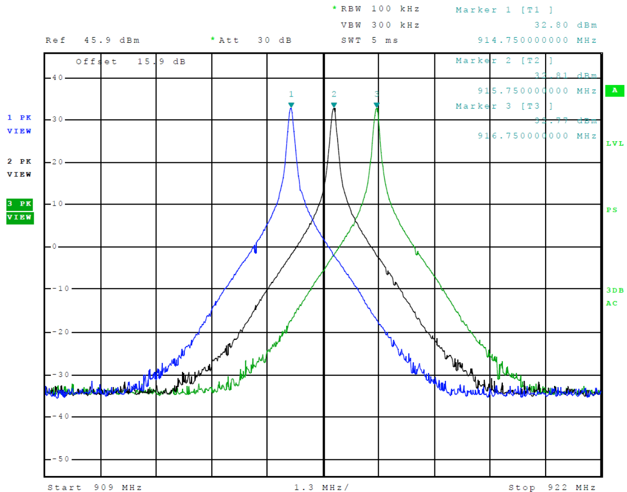
Figure 5 Transmitter Output Across Frequency Band IAG
