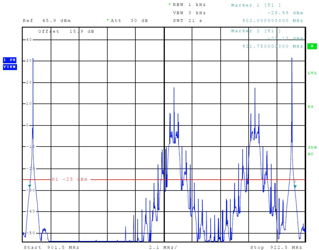
Figure 21 Emissions Mask Title 21
