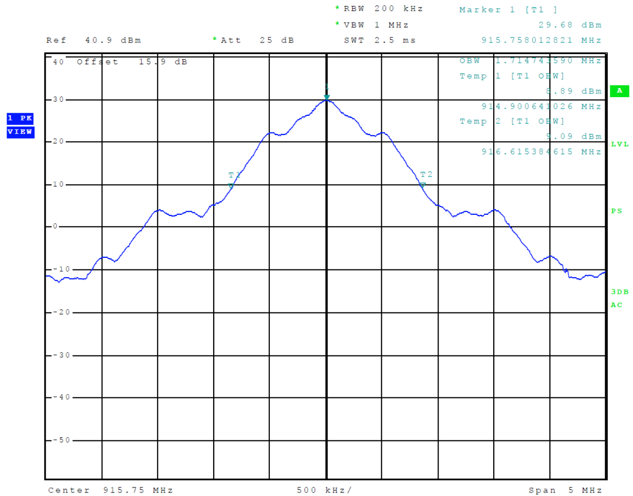
Figure 11 Occupied Bandwidth IAG, ASTM, CVS
