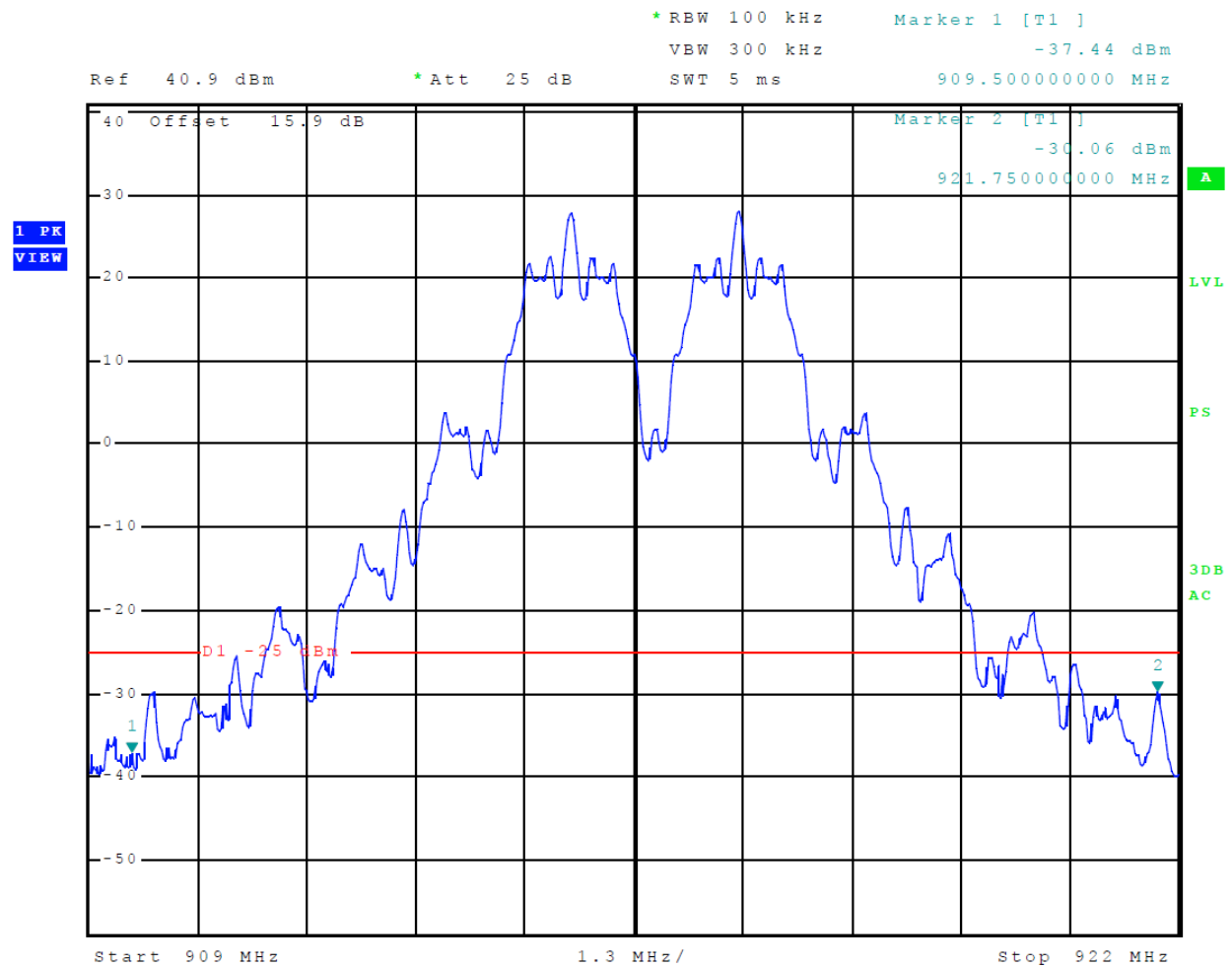
Figure 20 Emissions Mask Title 21
