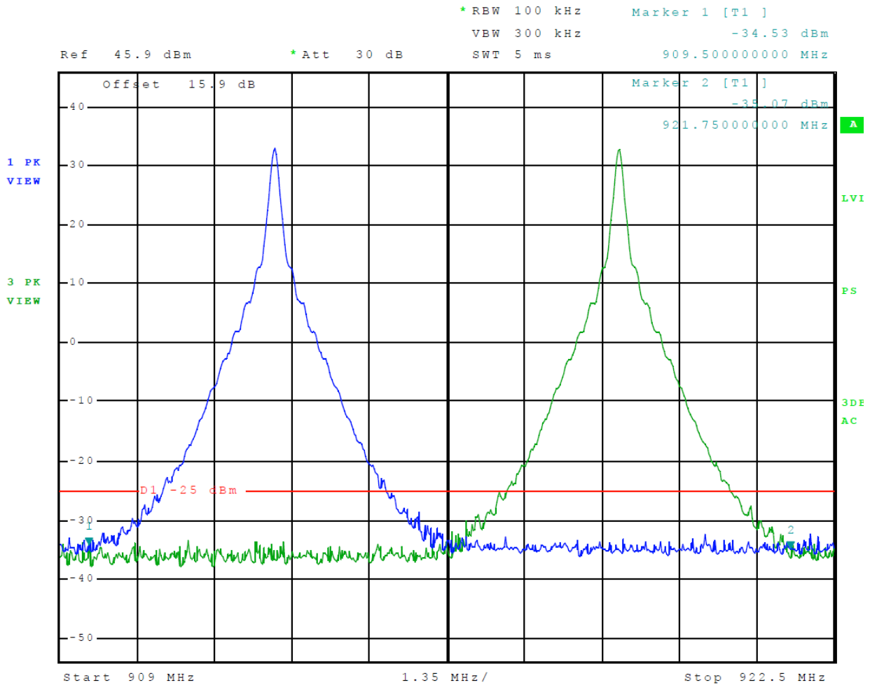
Figure 15 Emissions Mask EPC
