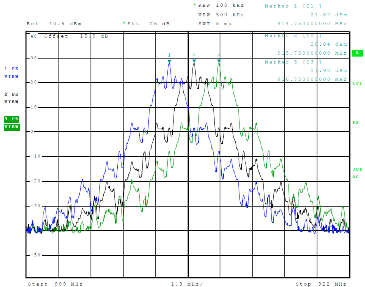
Figure 6 Transmitter Output Across Frequency Band ASTM
