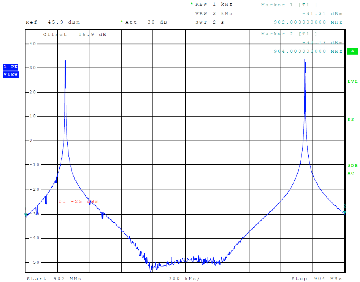
Figure 13 Emissions Mask ATA (CW)
