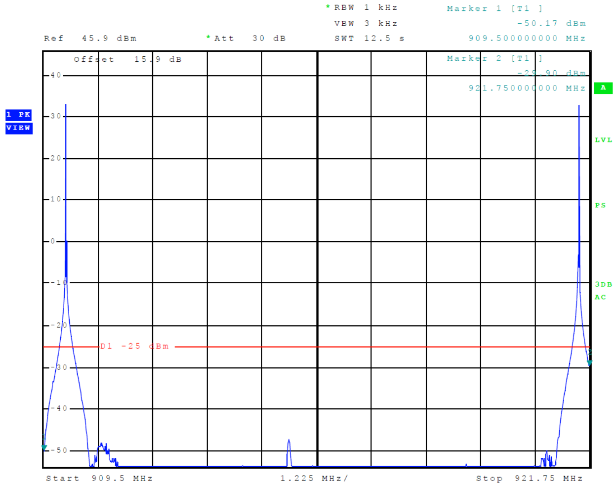
Figure 14 Emissions Mask CW (ATA)
