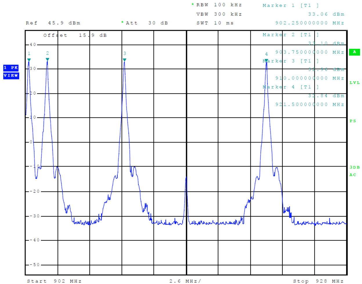
Figure 1 Transmitter Output Across Frequency Band CW (ATA) Highest Power Level
