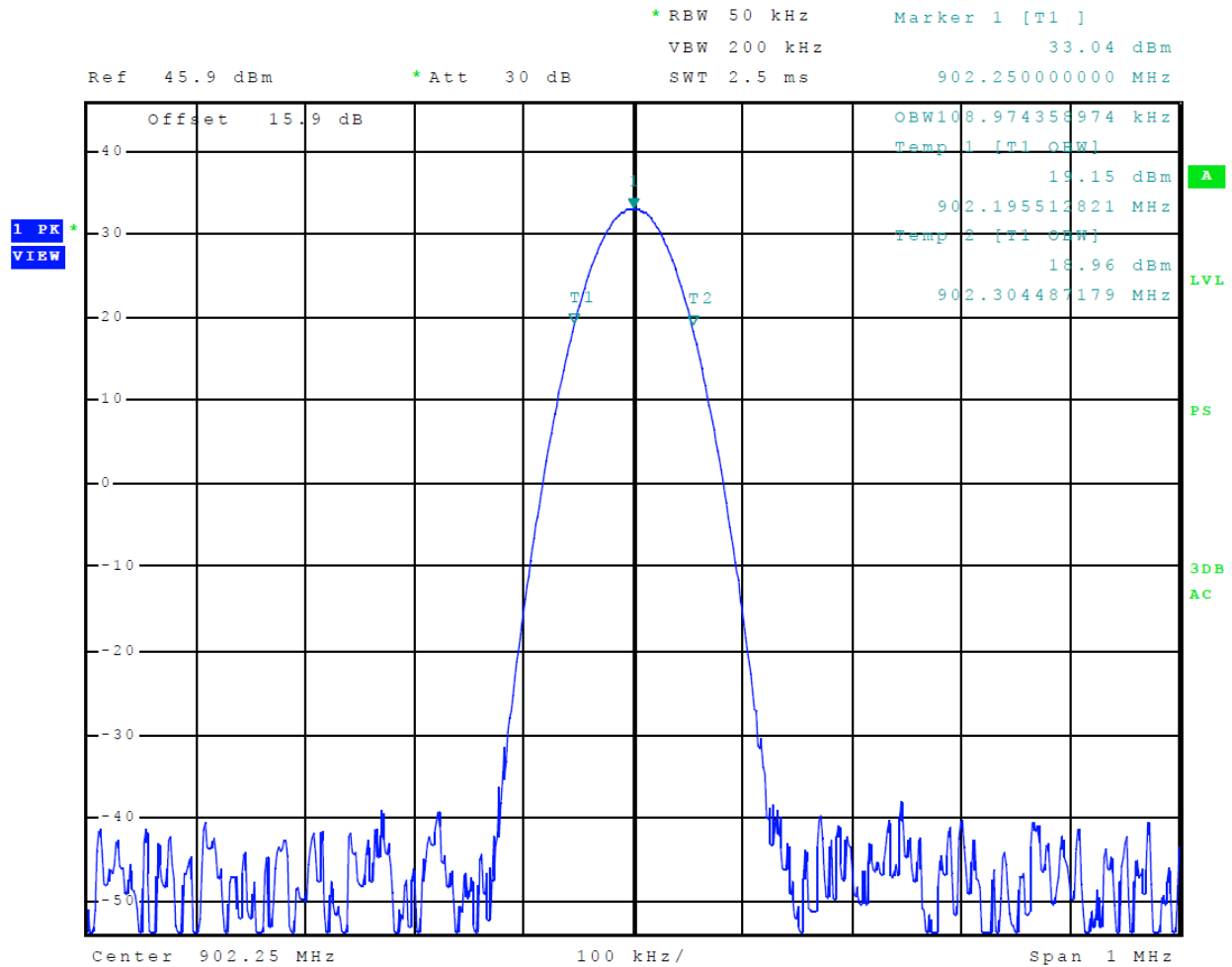
Figure 8 Occupied Bandwidth CW (ATA)
