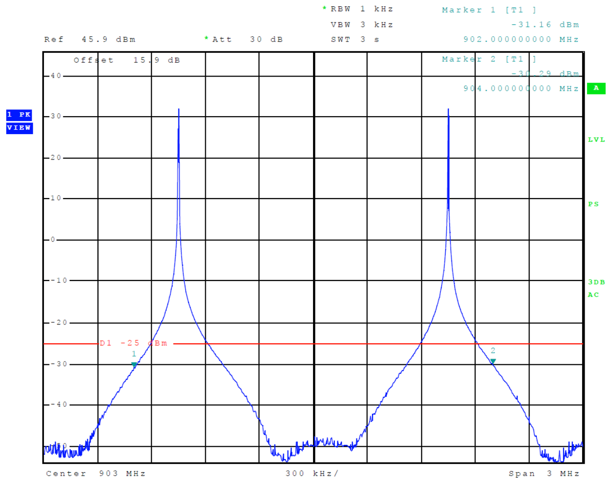
Figure 16 Emissions Mask SeGo
