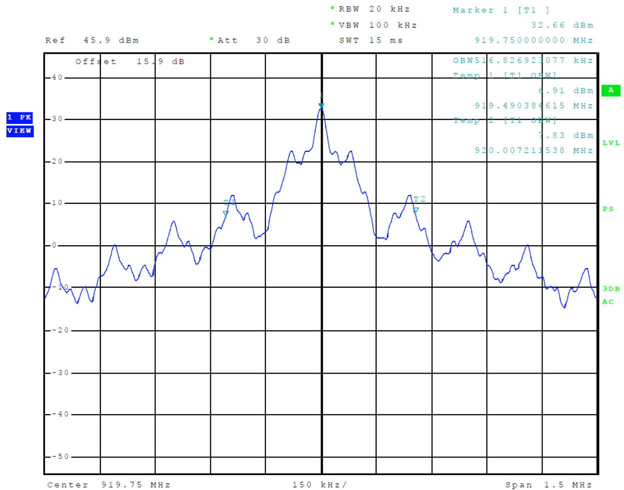
Figure 10 Occupied Bandwidth SeGo
