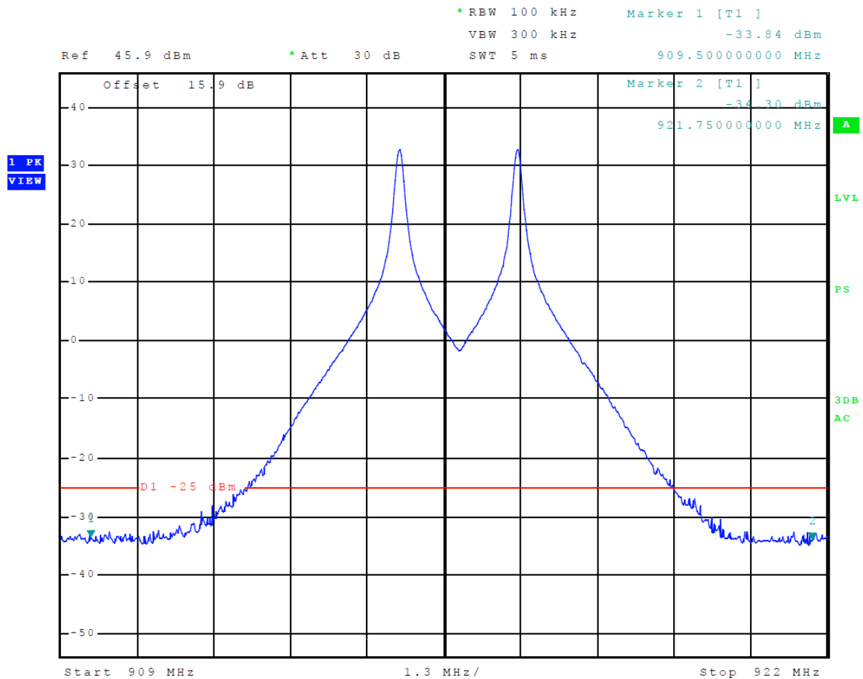
Figure 18 Emissions Mask IAG
