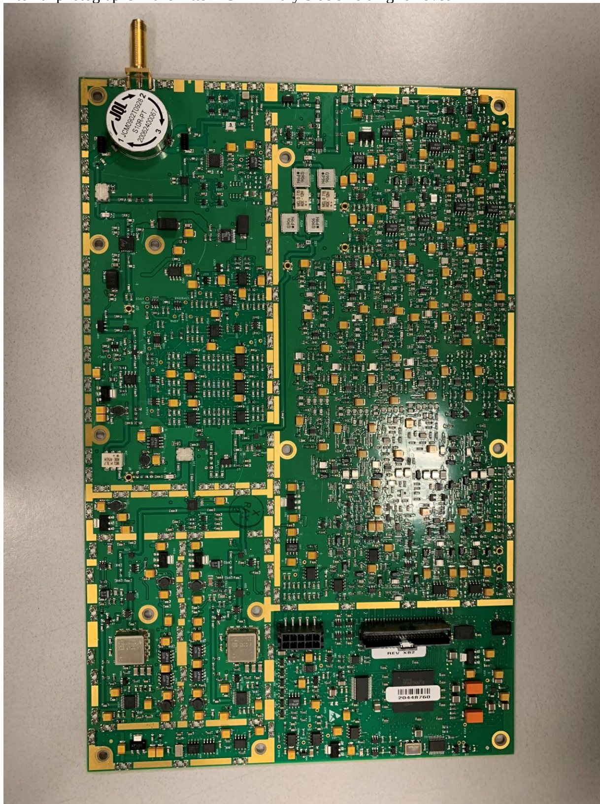
Internal photographs Transmitter PCB Primary Side shielding removed
