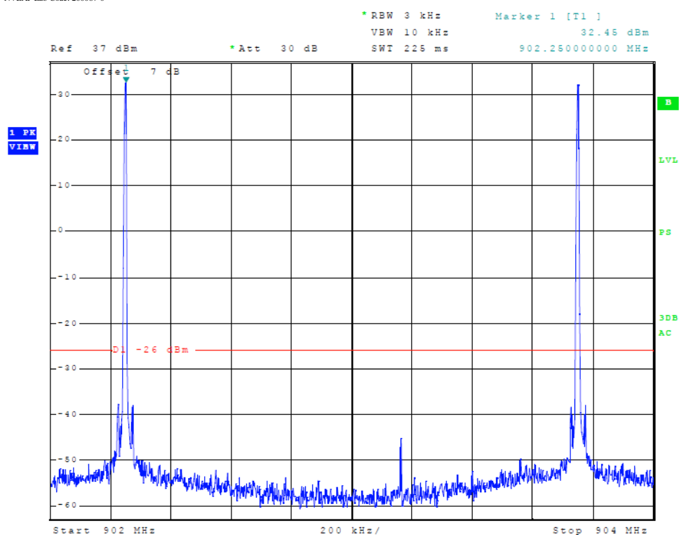
Figure 3 Emissions Mask (ATA, 902-904 MHz)
