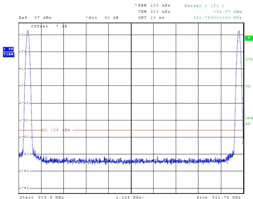
Figure 4 Emissions Mask (ATA, 909.5-921.75 MHz)
