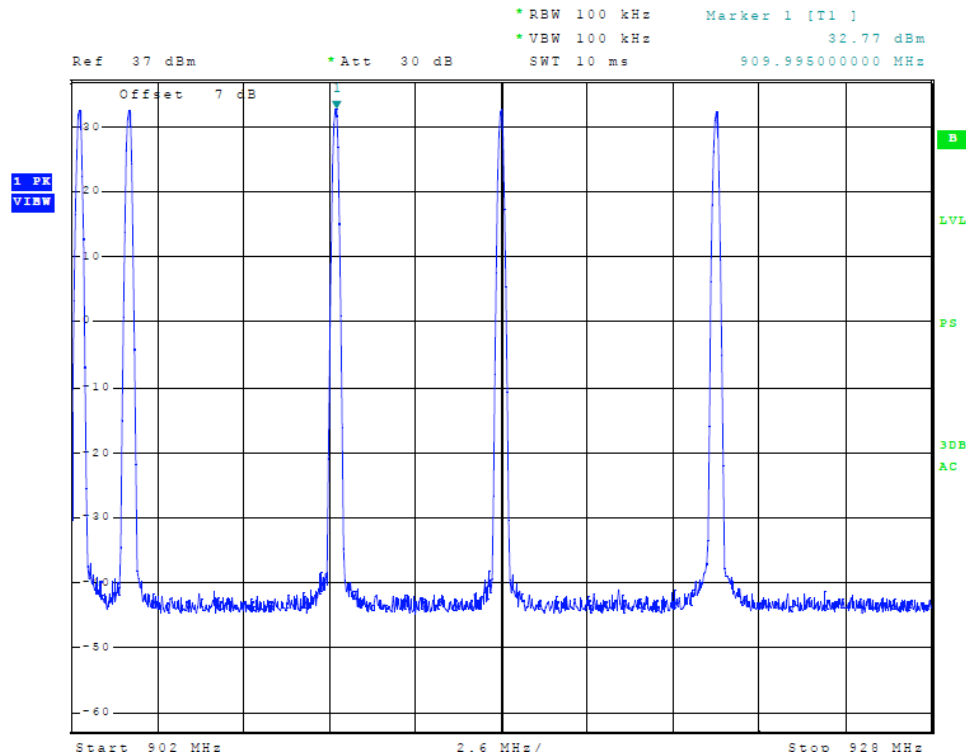
Figure 1 Transmitter Output across Frequency Band (Uplink)
