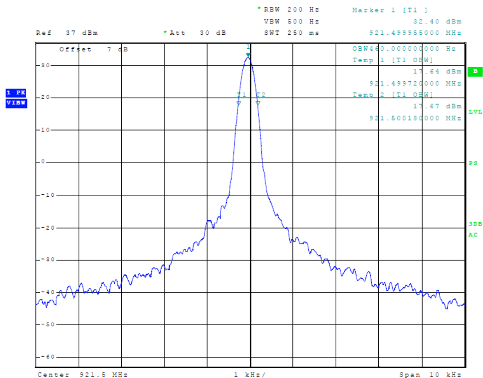
Figure 2 Occupied Bandwidth (ATA)
