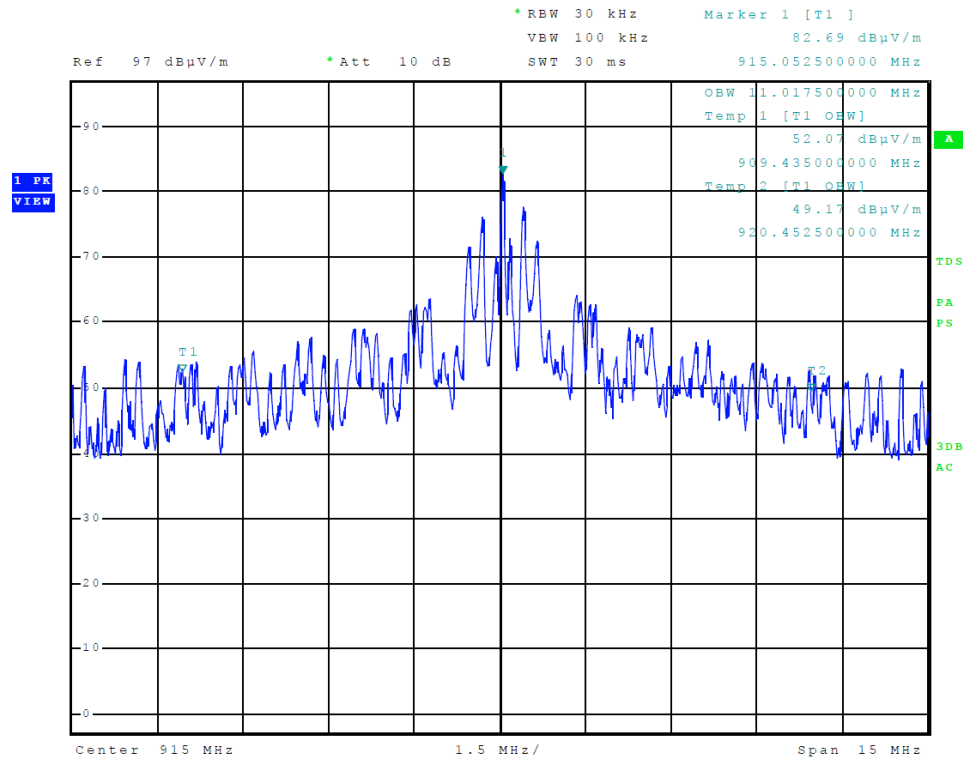
Figure 2 Occupied Bandwidth
