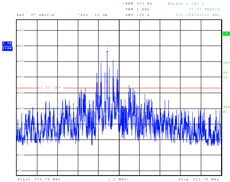
Figure 3 Emissions Mask
