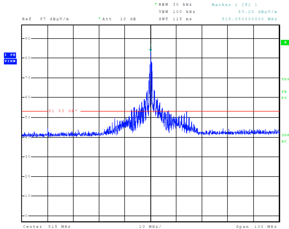
Figure 4 Emissions Mask
