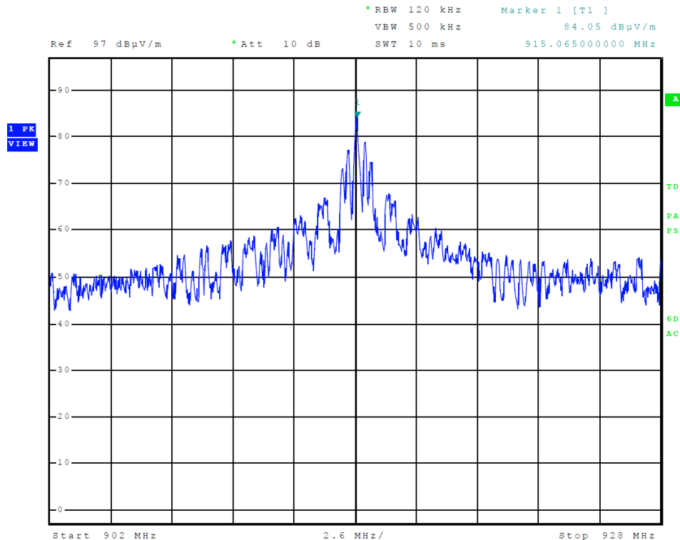
Figure 1 Transmitter Output across Frequency Band
