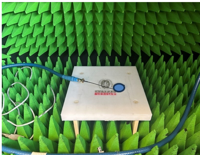
Photo of Maximum Conducted Output Power
