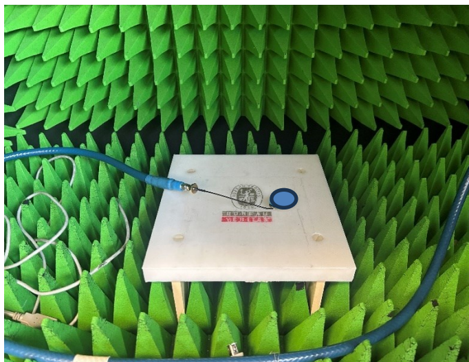
Photo of Unwanted emissions in non-restricted frequency bands
