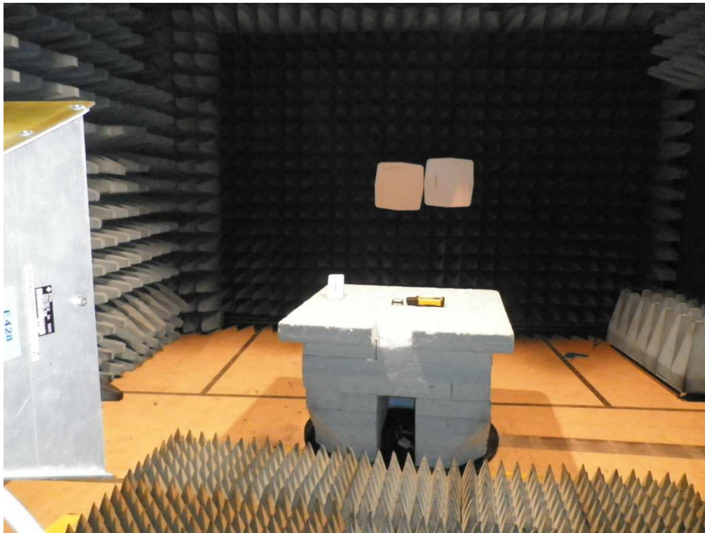
Semi-anechoic chamber above 1GHz set-up:
