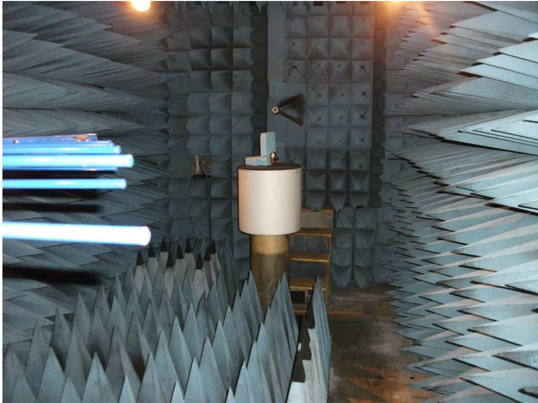
Photograph of the EUT as viewed from in front of the antenna, site Q.
