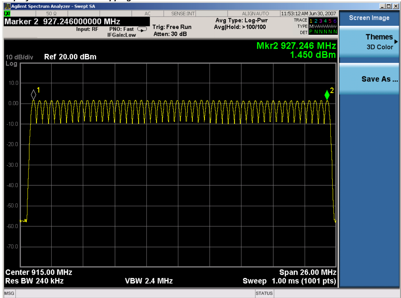
Plot 6-7. Number of Hopping Channels Plot – 50 Channels
