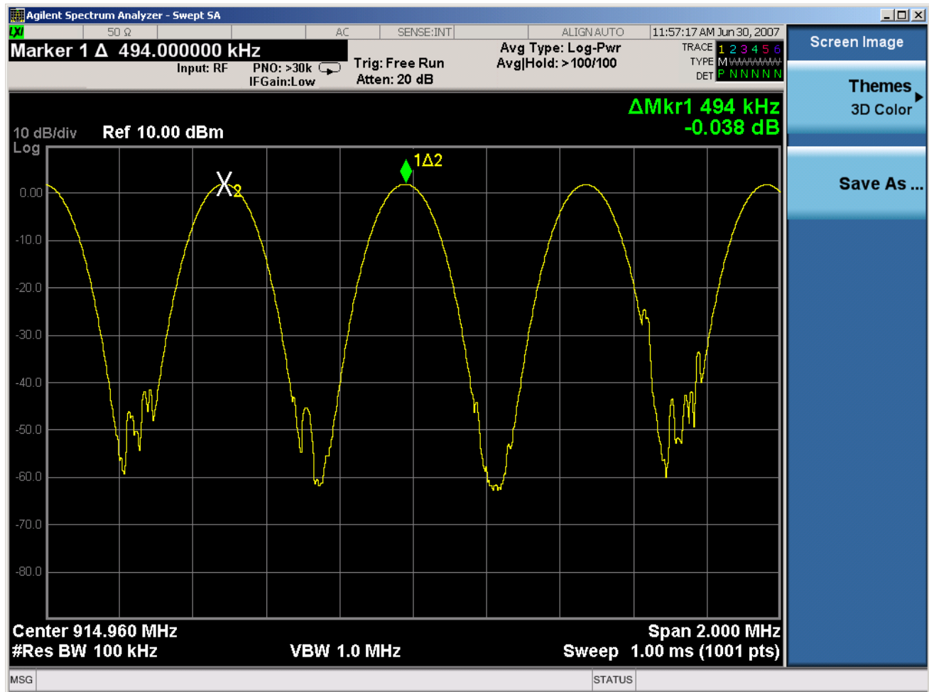
Plot 6-4. Channel Spacing Plot
