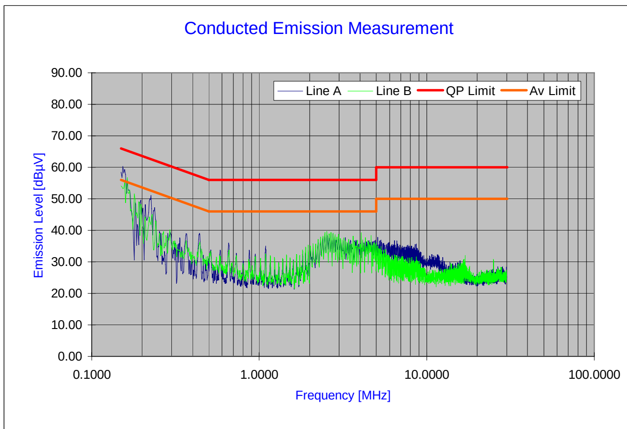
Plot 6-8. Line Conducted Plot
