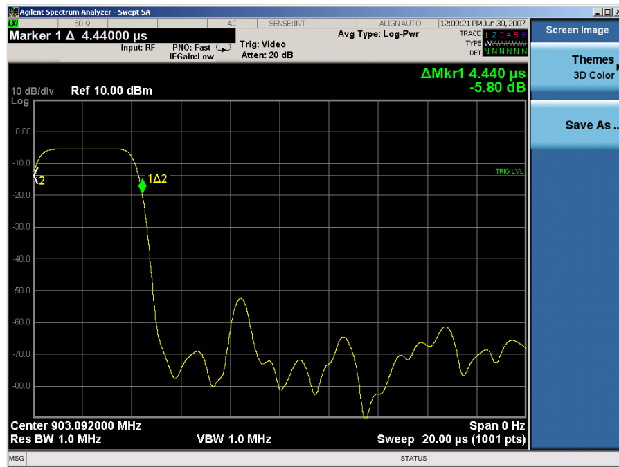
Plot 6-5. Time of Occupancy Plot
