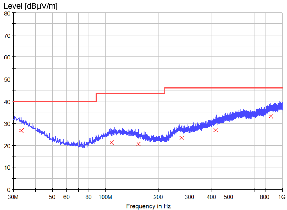
Figure 10: Spectral Diagrams, Radiated Emission, 30 MHz – 1000 MHz, Vertical polarization on mode 3
