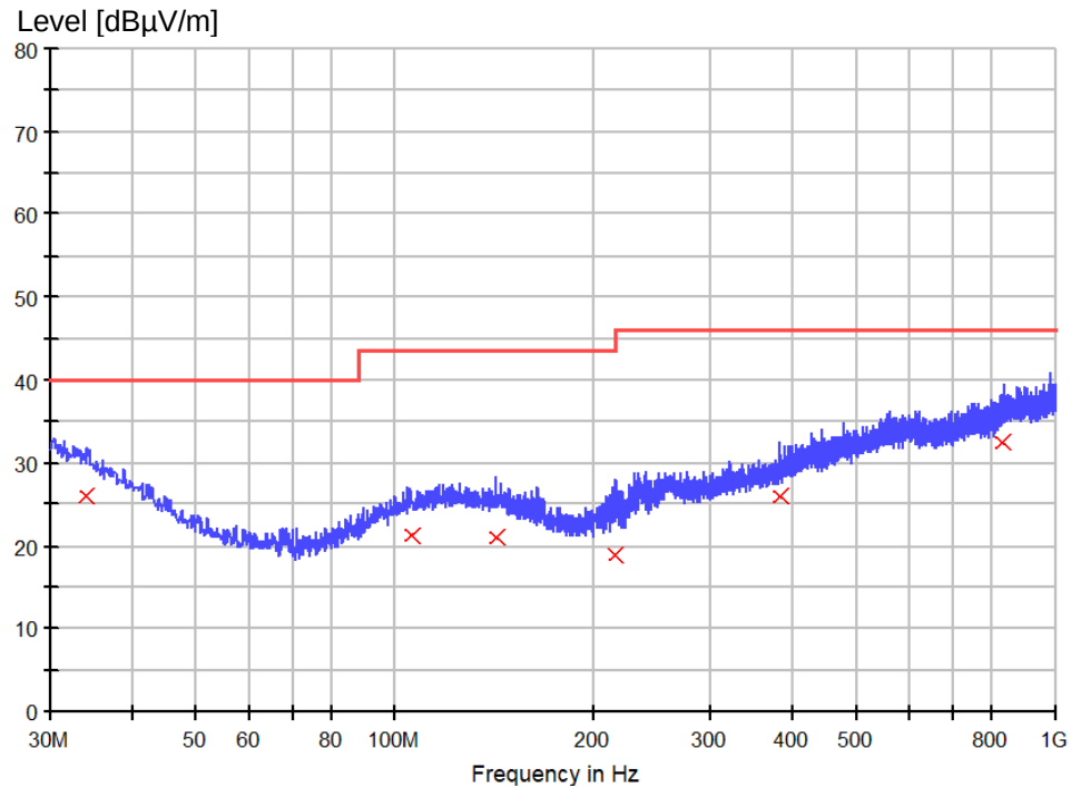
Figure 9: Spectral Diagrams, Radiated Emission, 30 MHz – 1000 MHz, Horizontal polarization on mode 3
