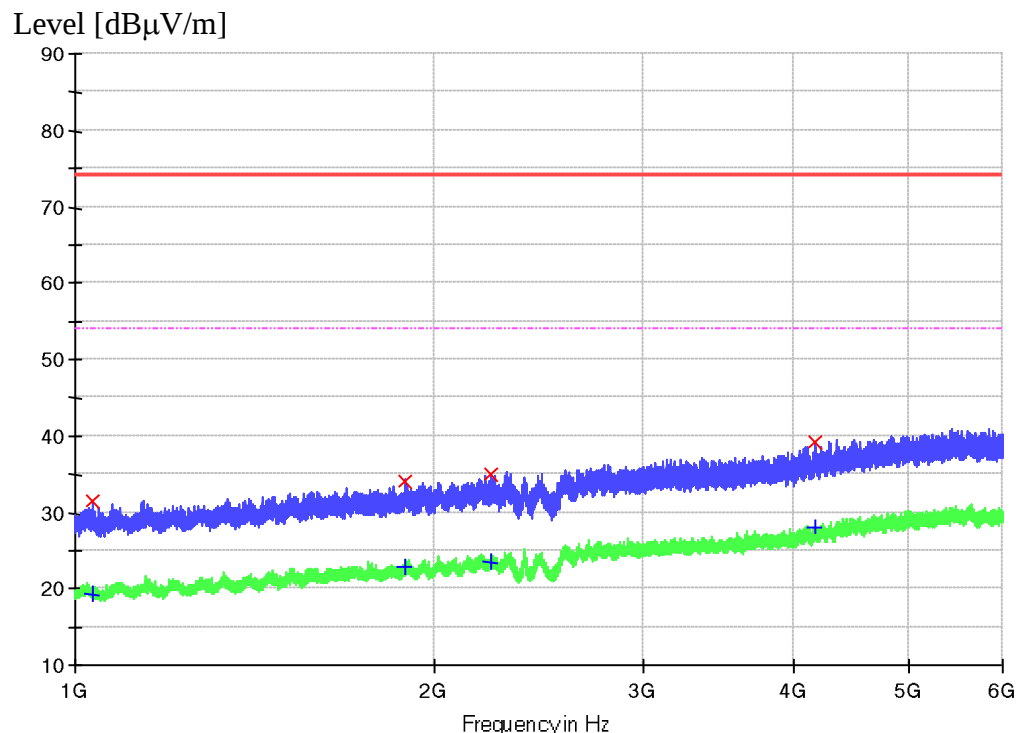
Figure 6: Spectral Diagrams and measurement results, 1-6 GHz, vertical polarization
