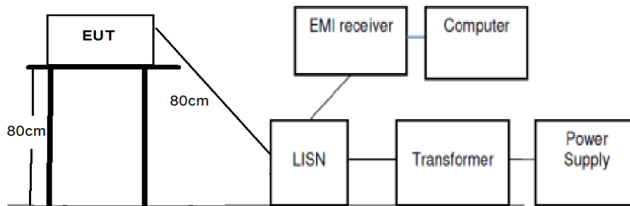
(Conducted emission)
