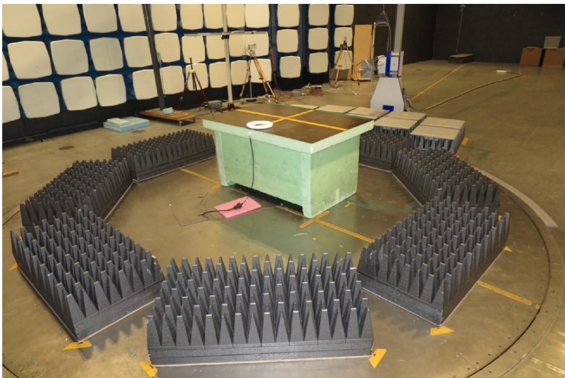
Test set up radiated emission 1 – 13 GHz
