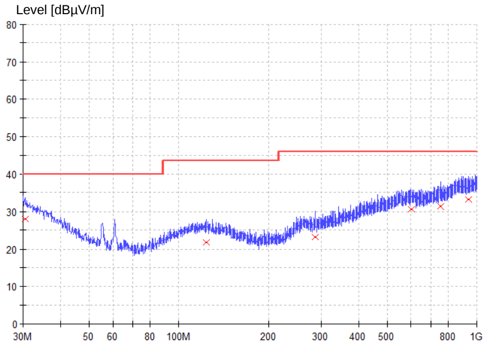
Figure 6: Spectral Diagrams, Radiated Emission, 30 MHz – 1000 MHz, Vertical polarization, Mode 1
