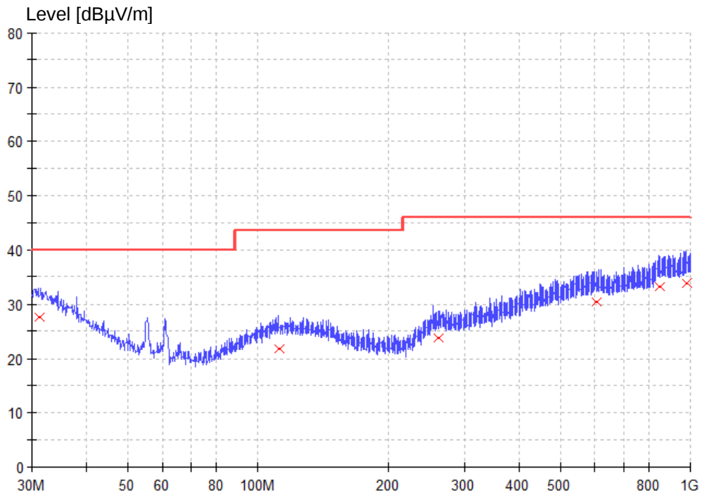
Figure 8: Spectral Diagrams, Radiated Emission, 30 MHz – 1000 MHz, Vertical polarization, Mode 2
