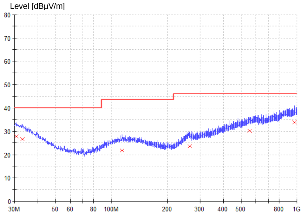
Figure 7: Spectral Diagrams, Radiated Emission, 30 MHz – 1000 MHz, Horizontal polarization, Mode 2
