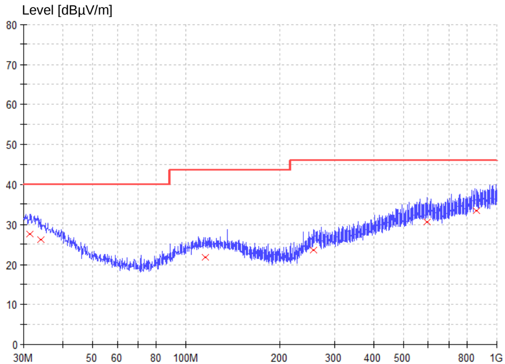
Figure 5: Spectral Diagrams, Radiated Emission, 30 MHz – 1000 MHz, Horizontal polarization, Mode 1
