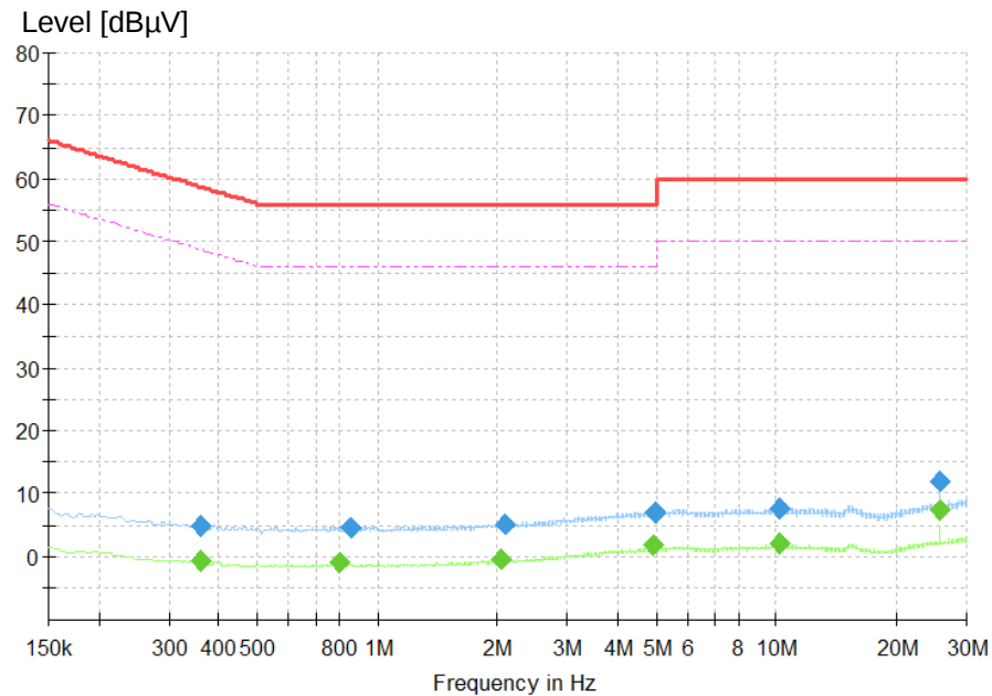
Figure 2: Spectral Diagrams, Conducted Emission, 150 kHz – 30 MHz, N
