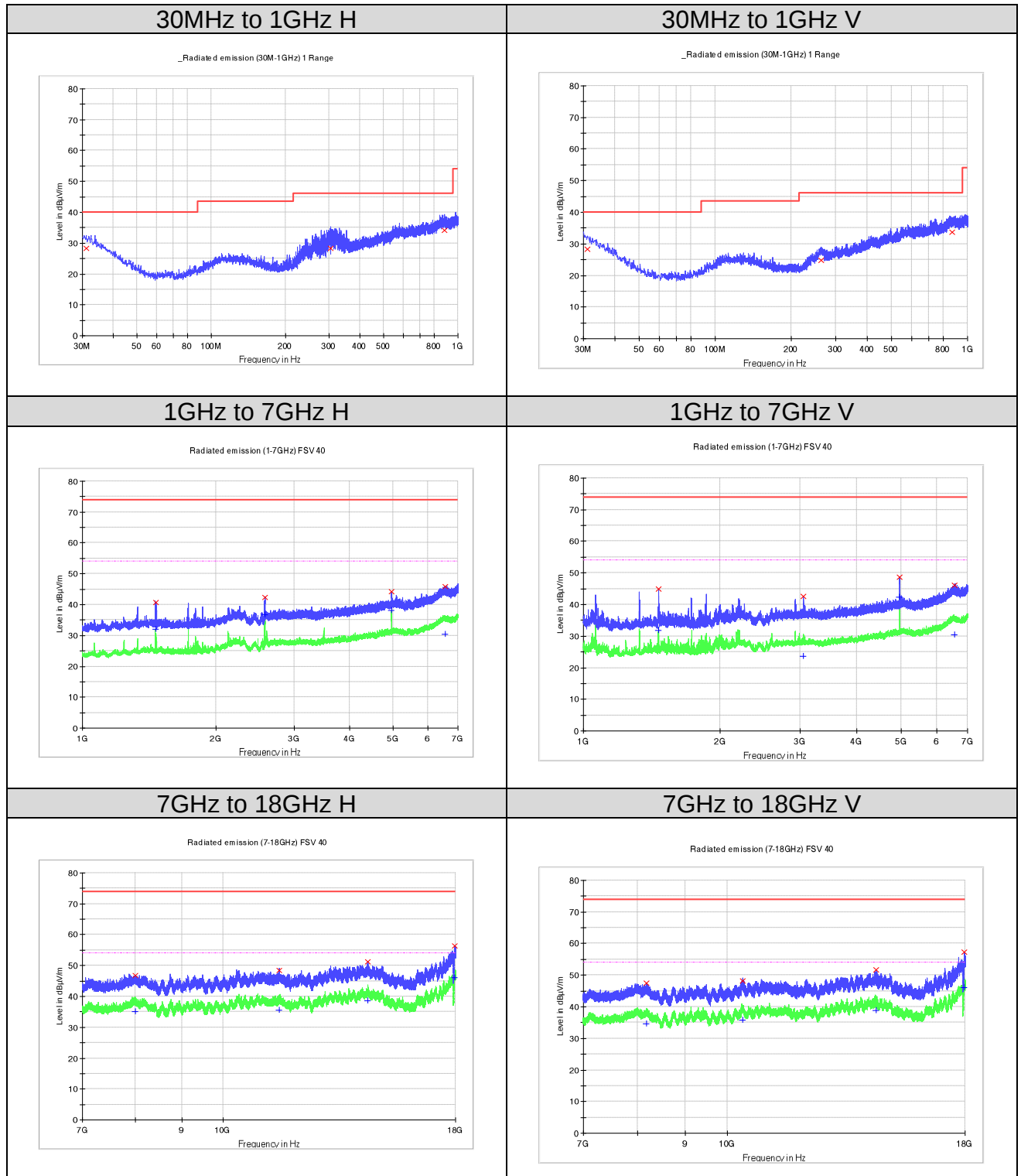
Figure 11: Radiated Spurious Emission, 2480MHz
