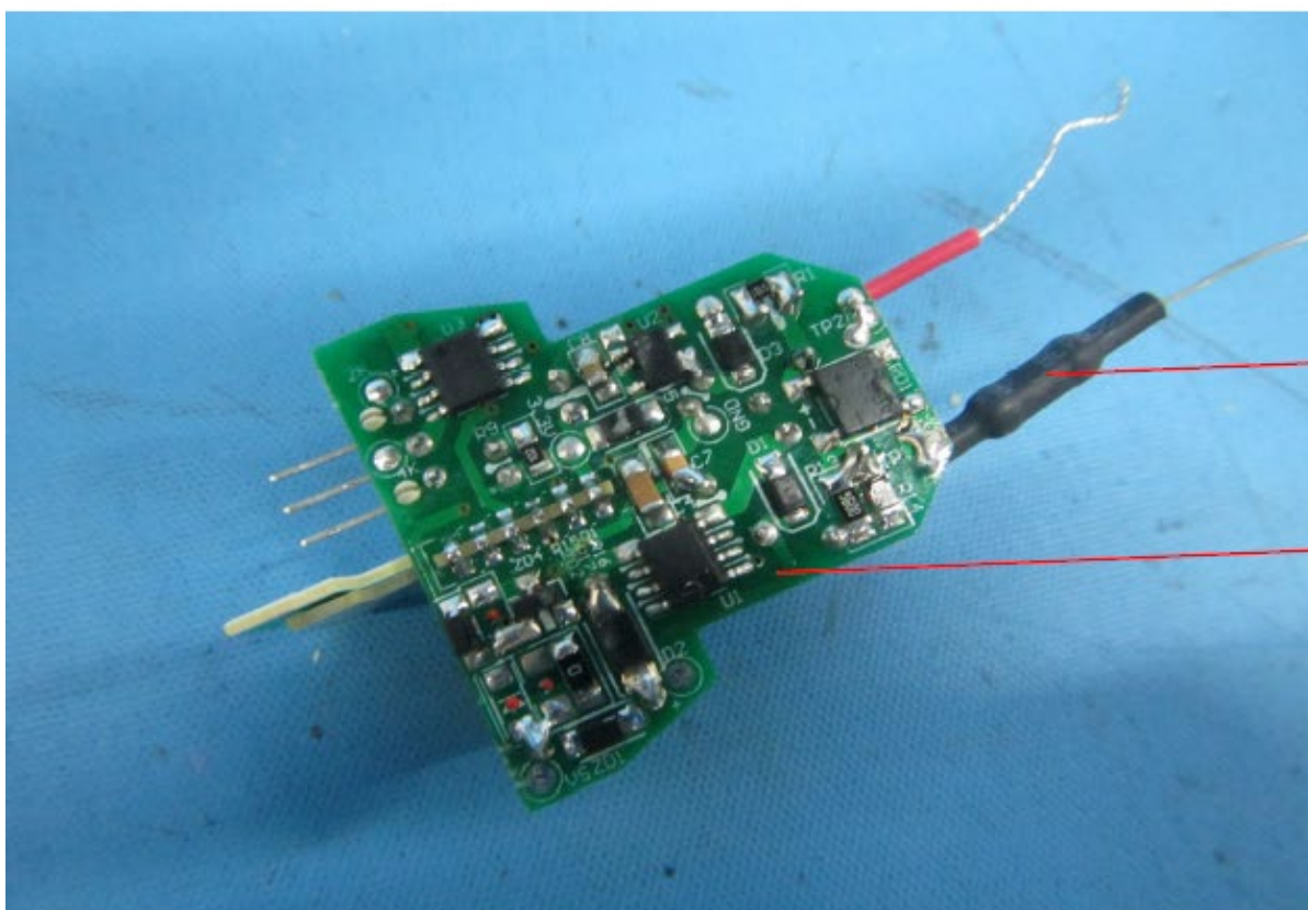
Photo 8 - Internal view
