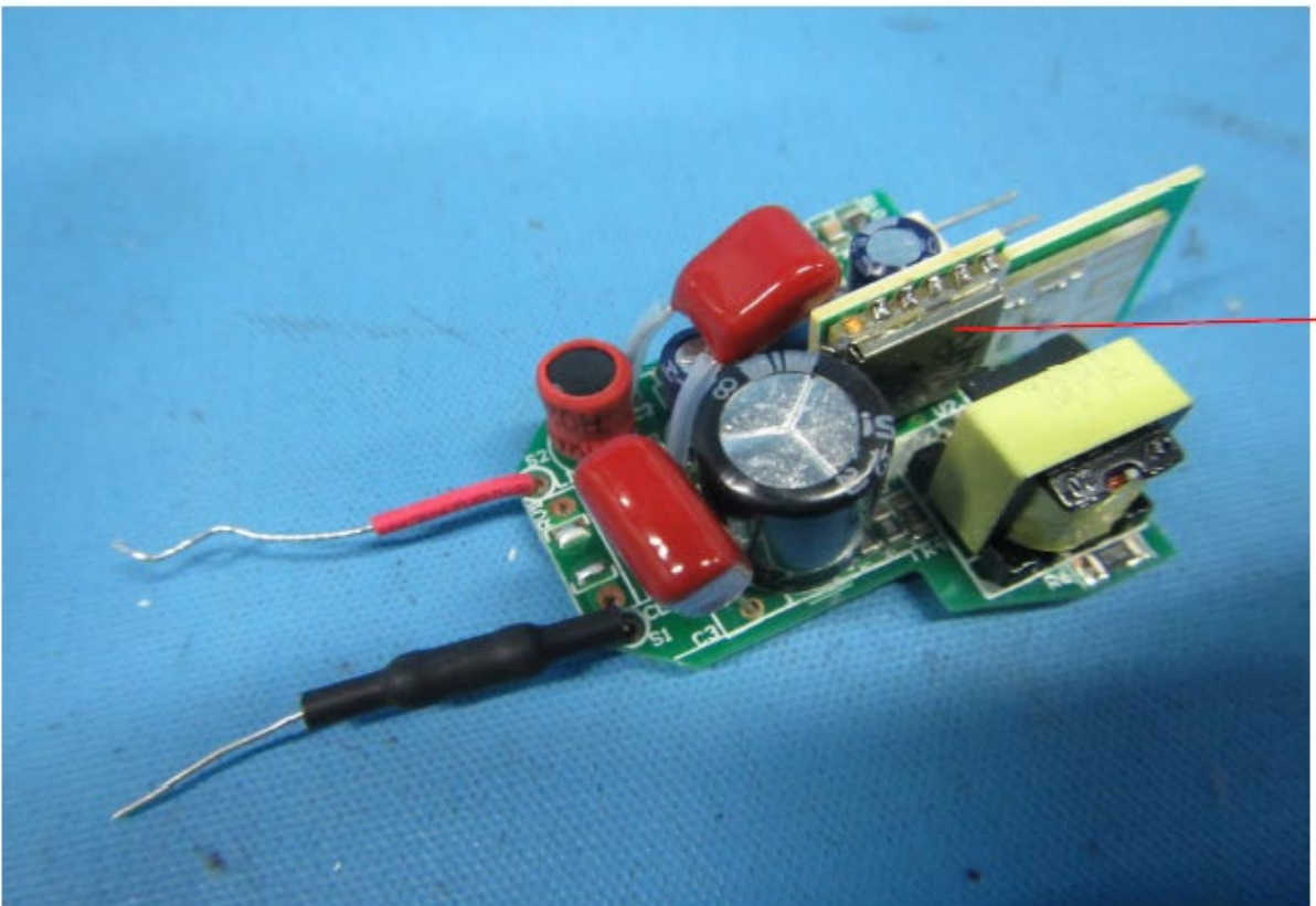
Photo 6 - Internal view
