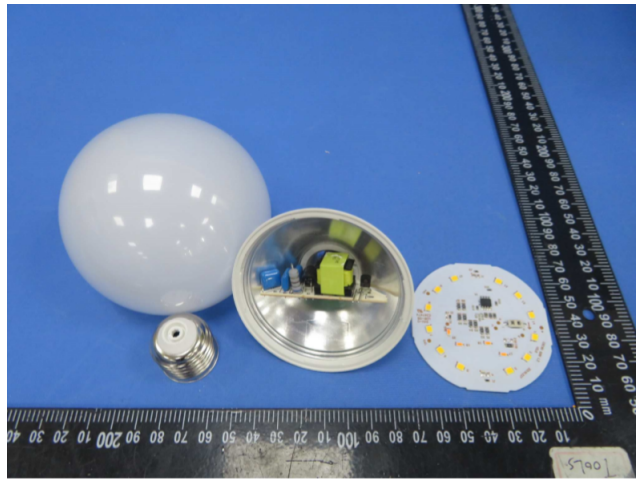
Exploded view
