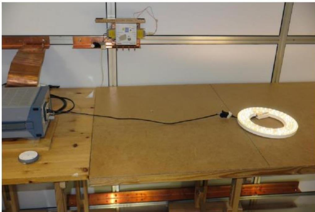
Photo of the test set-up for conducted emission
