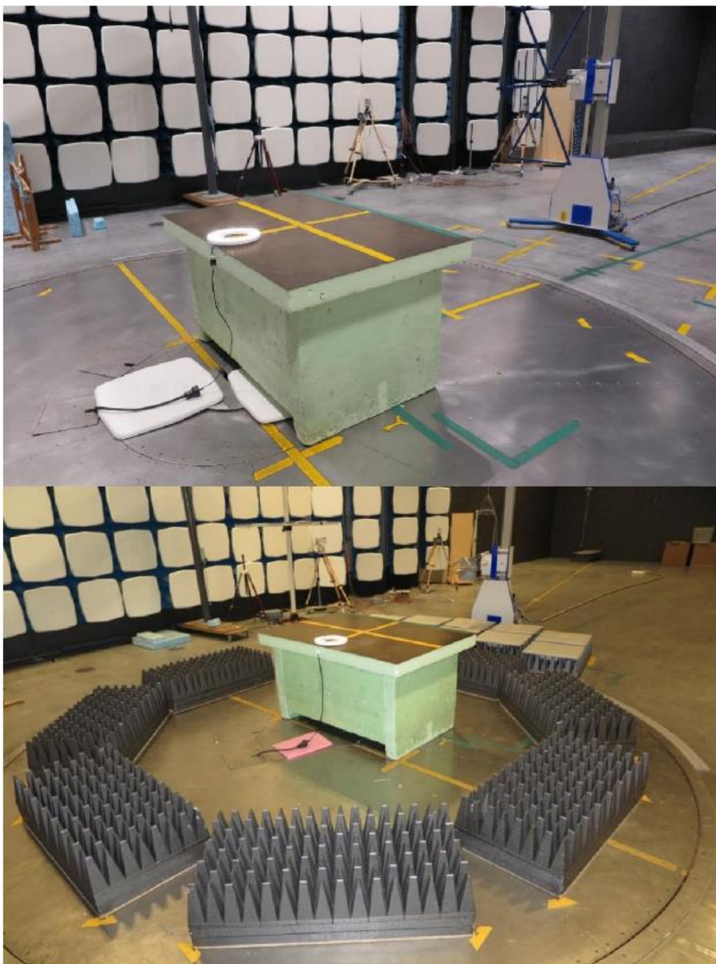
Photo of the test set-up for radiated emission
