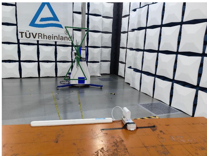
Photograph 4: Set-up for measurement of radiated emission, Mode 3
