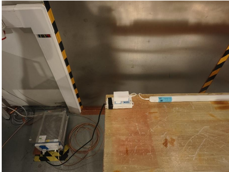
Photograph 2: Set-up for measurement of conducted emission, Mode 2
