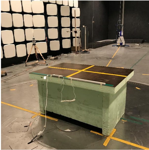
Test set up radiated emission 30 MHz – 1 GHz, 10W
