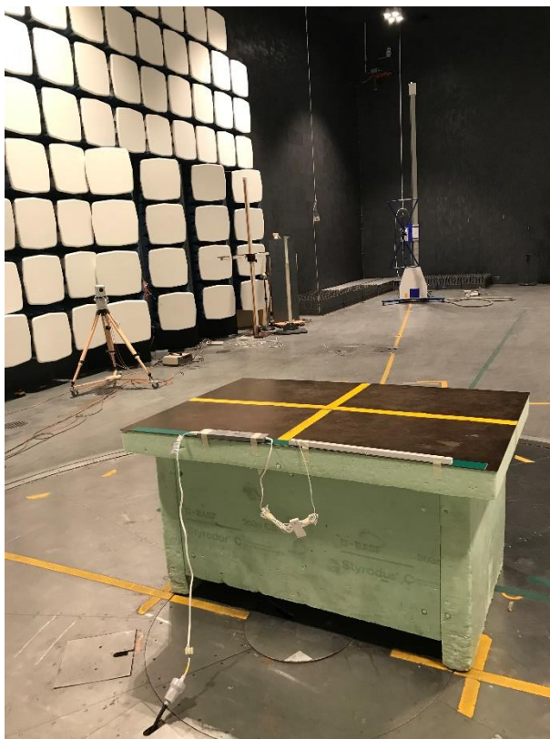
Test set up radiated emission 30 MHz – 1 GHz, 30W
