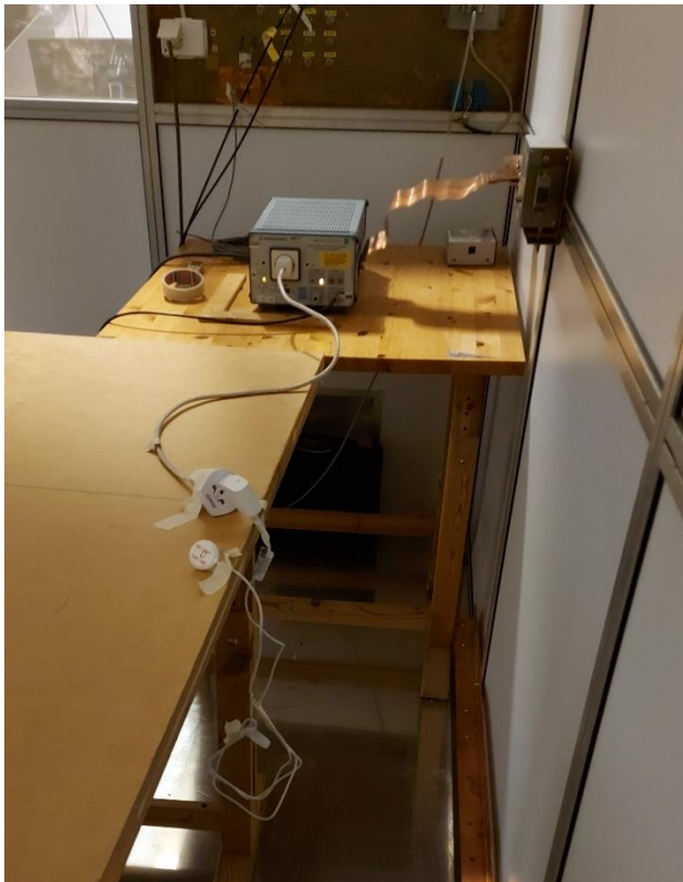
Test setup for conducted emission 150 kHz – 30 MHz
