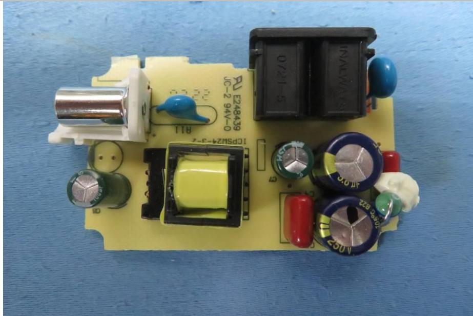
PCB View for adapter
