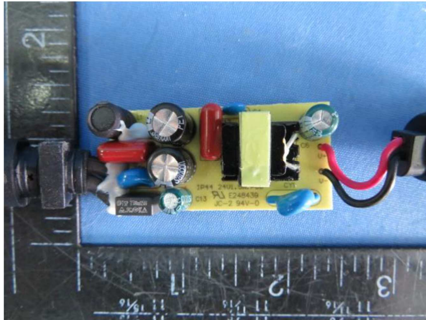
Power unit ICPSL24-2-IL-1 PCB view for all models
