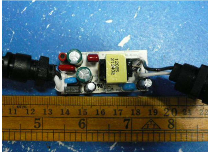
Power unit ICPSW24-3.6-IL-1 PCB view for all models
