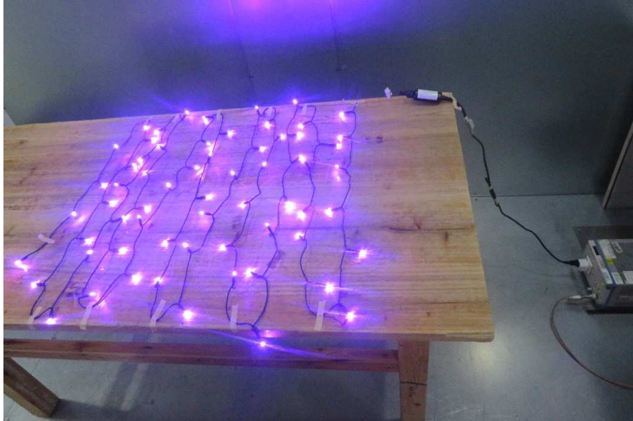
Conducted Emission
