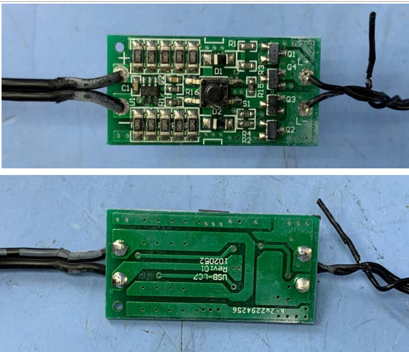
Controller PCB view
