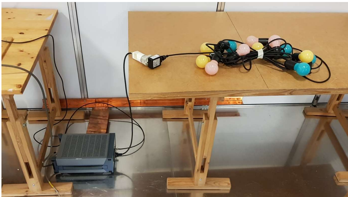
Test setup for conducted emission 150 kHz – 30 MHz
