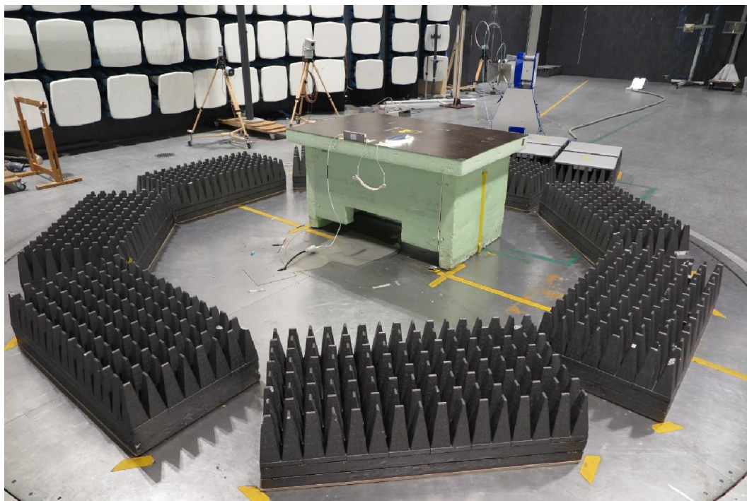
Test set up radiated emission 1 GHz – 13 GHz
