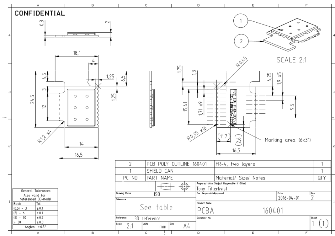
Figure 2 - Physical dimensions of the ICC-1 module
