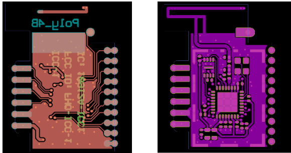
Figure 1 - Silkscreen printing from bottom and top view
