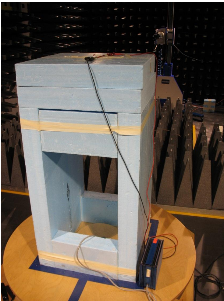
Test set up radiated emission preview sweeps 13 – 18 GHz, test site 'Wireless chamber'
