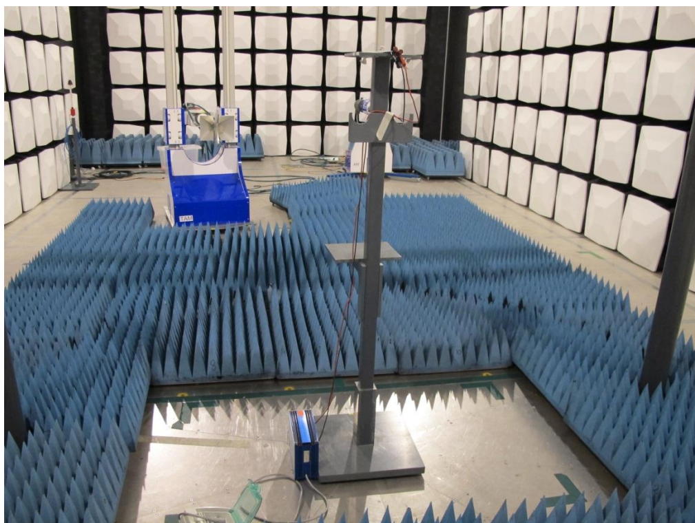
Test set up radiated emission 1 – 13 GHz, test site '5m Chamber'
