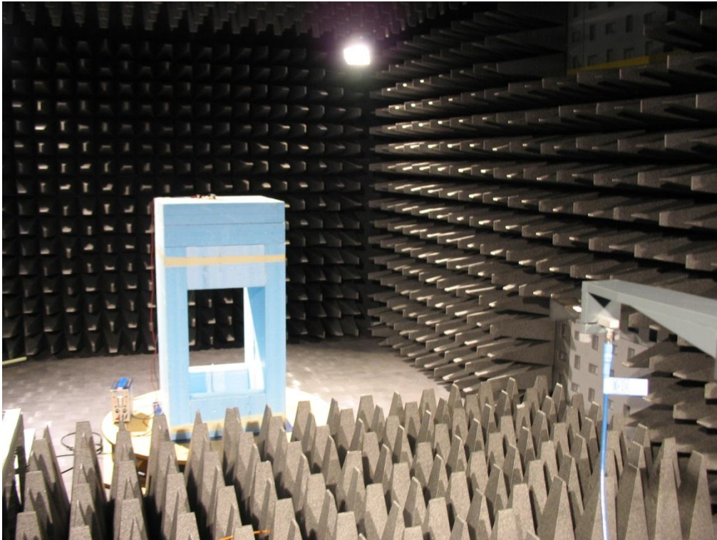
Test set up radiated emission preview sweeps 18 – 26.5 GHz, test site 'Wireless chamber'
