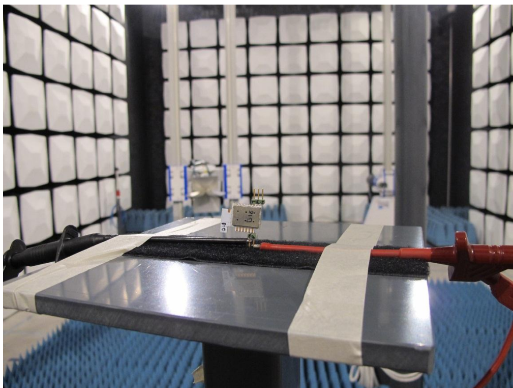
EUT in position X
