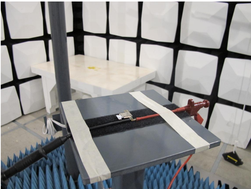
EUT in position Z
