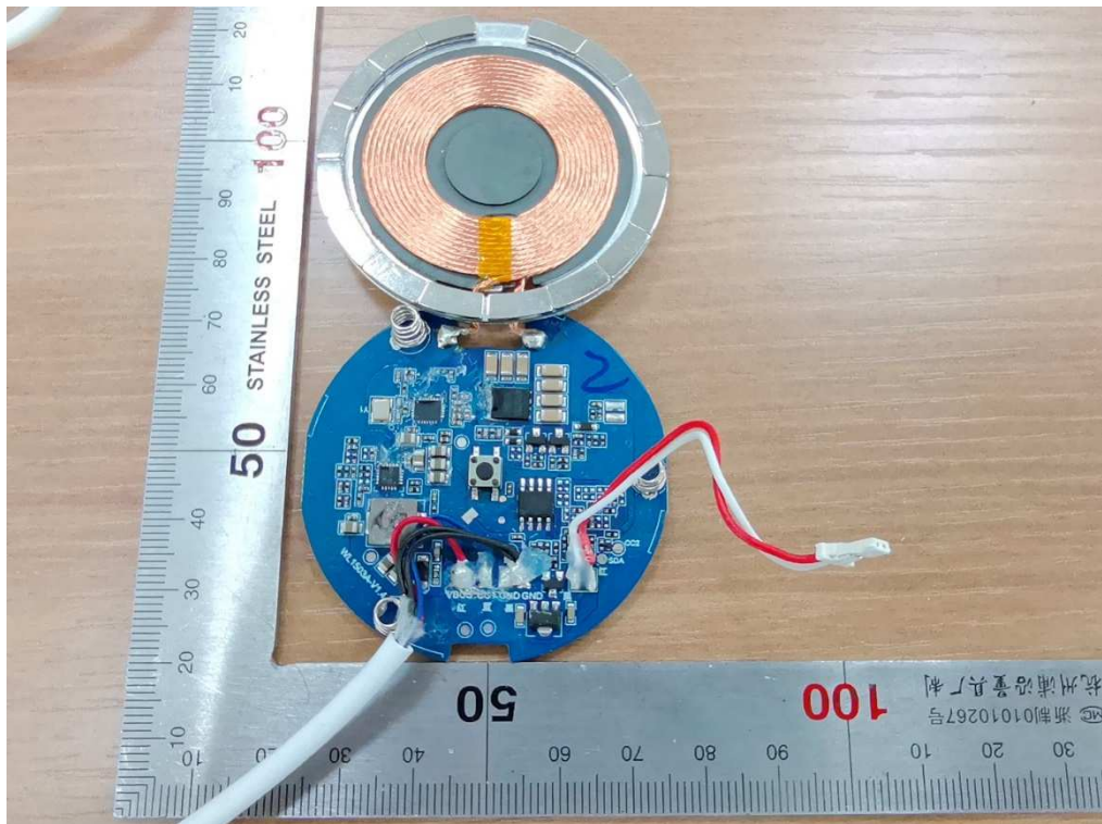
Bild / Picture 4: Coil with PCB
