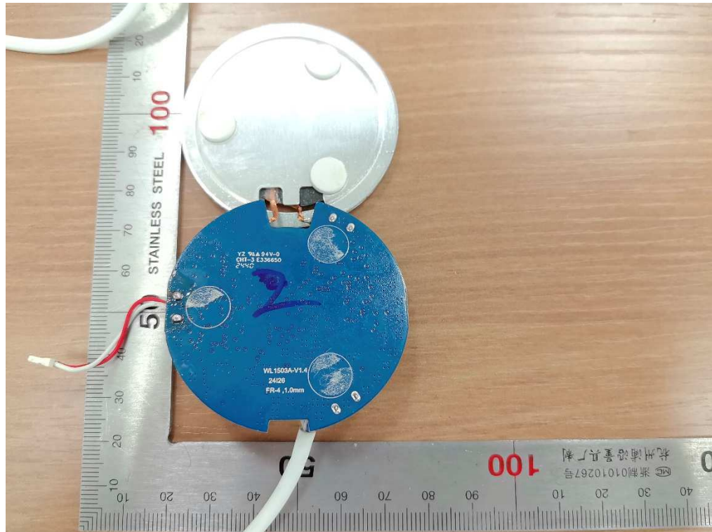
Bild / Picture 6: LED PCB view
