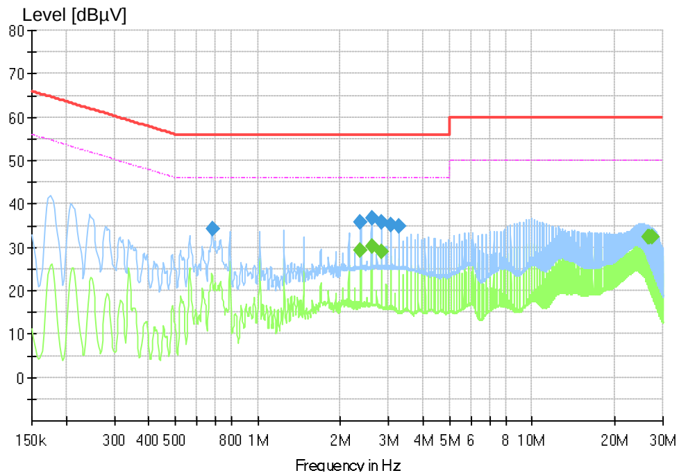
Figure 4: Spectral Diagrams, Conducted Emission, 150 kHz – 30 MHz, N, 5 W load
