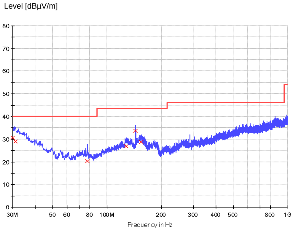
Figure 8: Spectral Diagrams and measurement results, vertical polarization (30 MHz to 1 GHz), 5 W load
