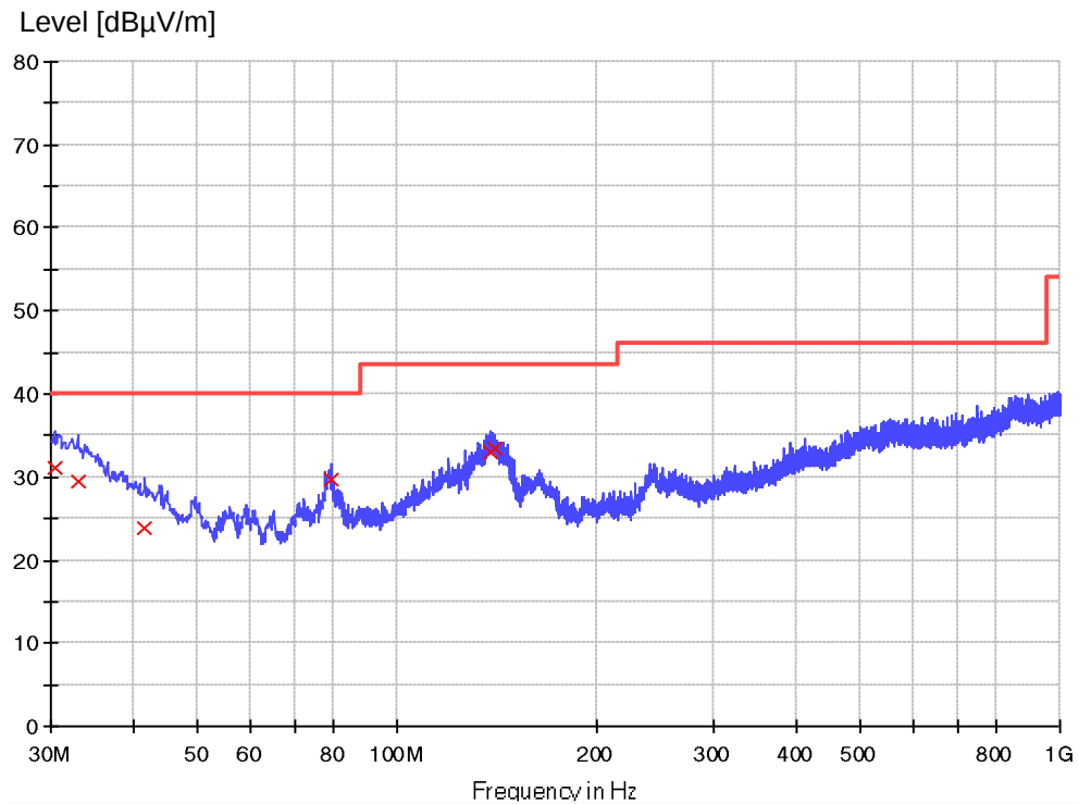
Figure 6: Spectral Diagrams and measurement results, vertical polarization (30 MHz to 1 GHz), 15 W load
