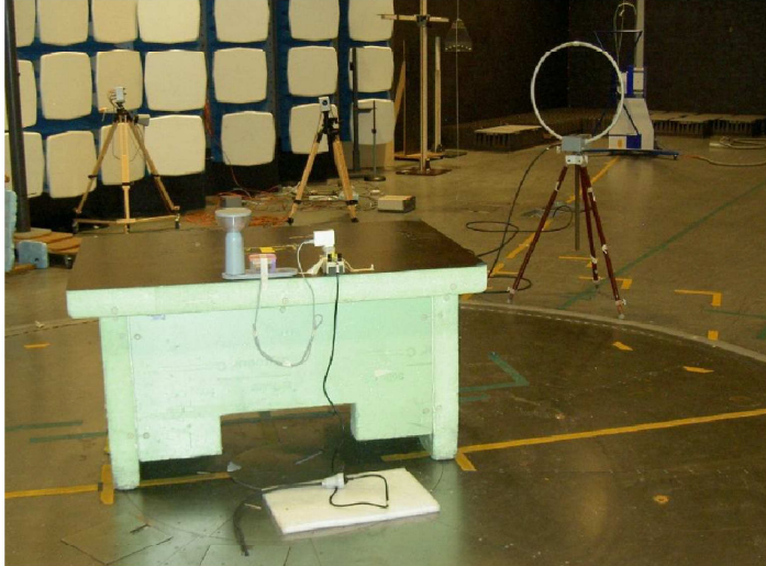
Test set up radiated emission, loop antenna 9 kHz – 30 MHz
