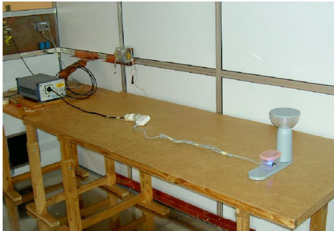
Test setup for conducted emission 150 kHz – 30 MHz
