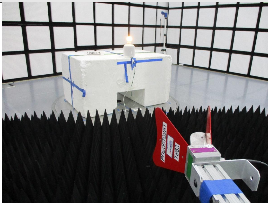
Photo of test setup for Radiated Emissions: 1 GHz -18 GHz
