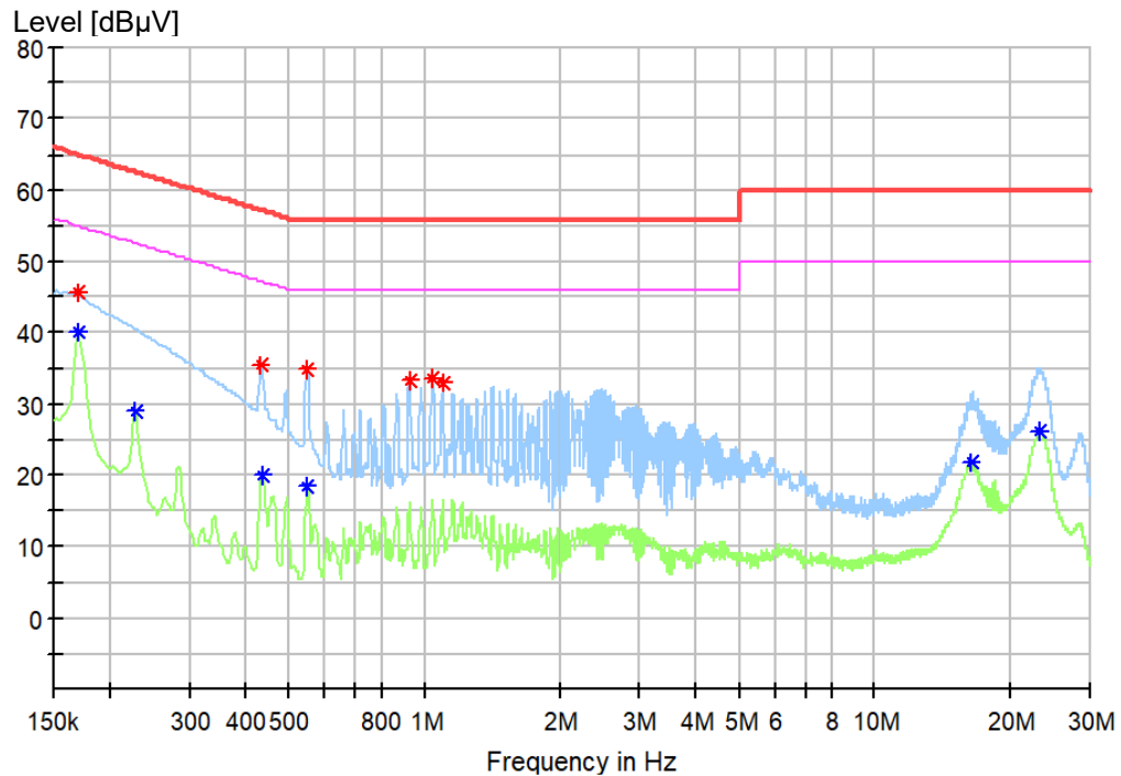
Figure 1: Spectral Diagrams, Conducted Emission, 150 kHz – 30 MHz, L
