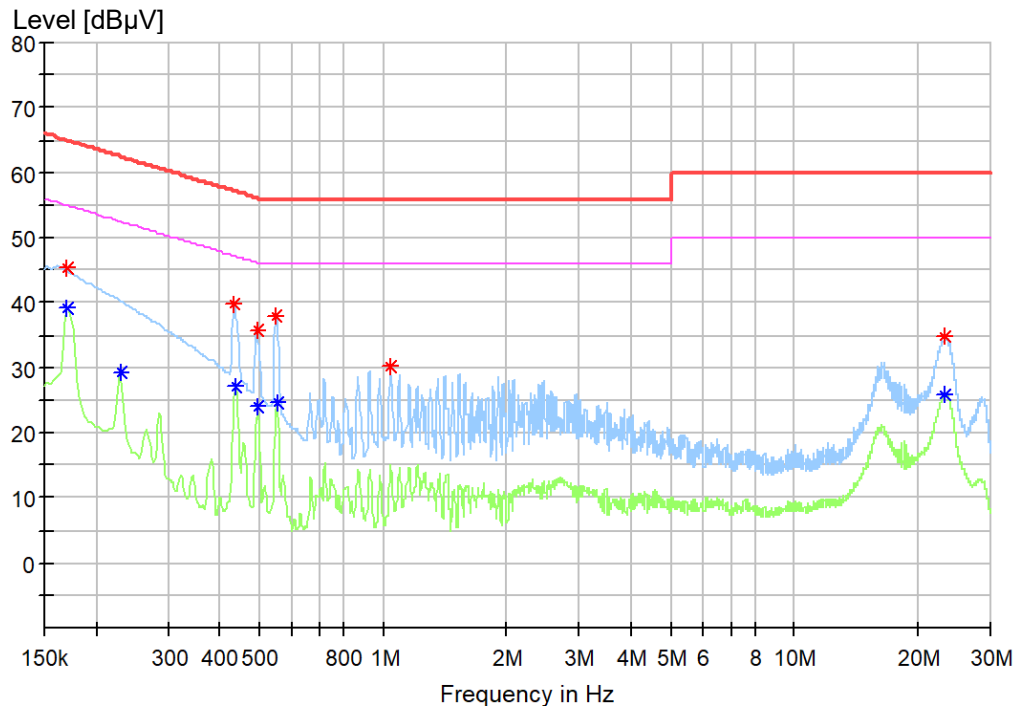
Figure 2: Spectral Diagrams, Conducted Emission, 150 kHz – 30 MHz, N
