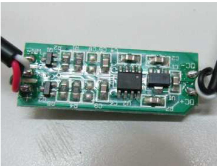
3d) Switch (Switch board back)
