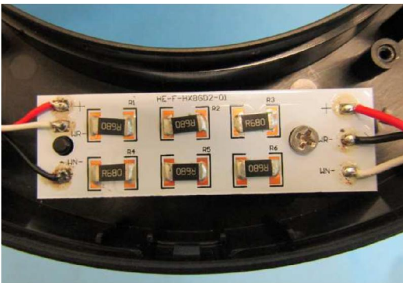
2c) Resistor board (Front)
