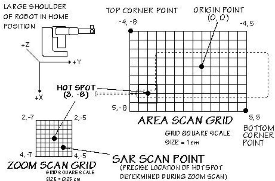
Figure 6. SAR Measurement Points in Area Scan and Zoom Scan Grids Showing the Typical Hot Spot with respect to the Phone
