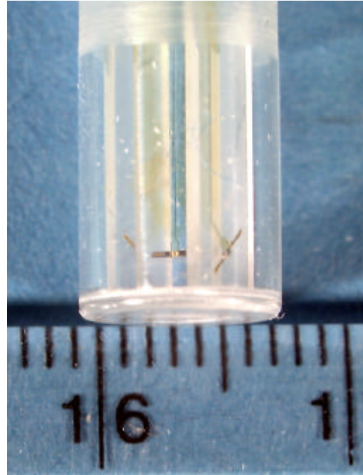
Figure 3. Isotropic E-field Probe
