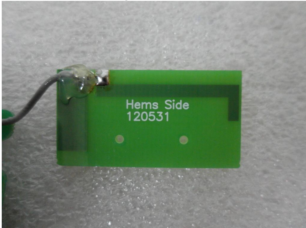
Zigbee Antenna 2
