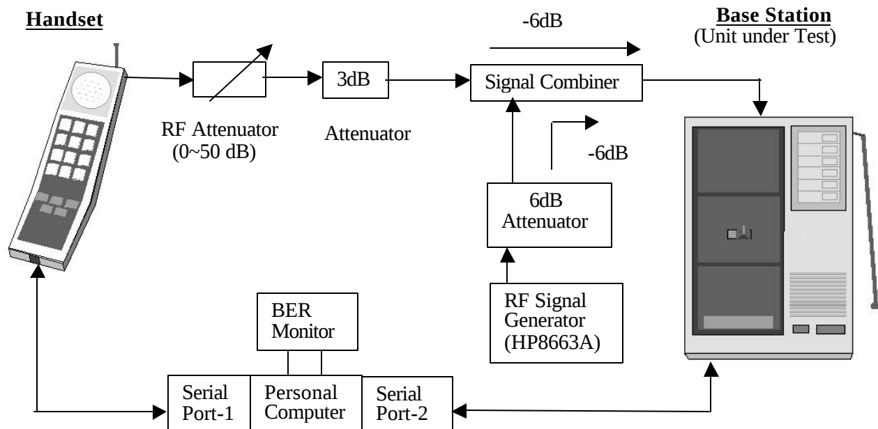
Figure 1: Test Setup
