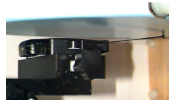
Figure 18. Body SAR Test
