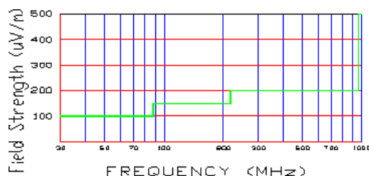
Figure 10. Harmonic Limits at 3 meters
