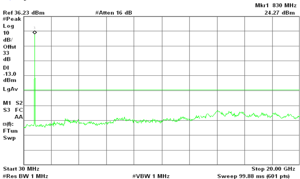
Figure 12-1: Out of Band emission at antenna terminals – HSDPA CH Low
