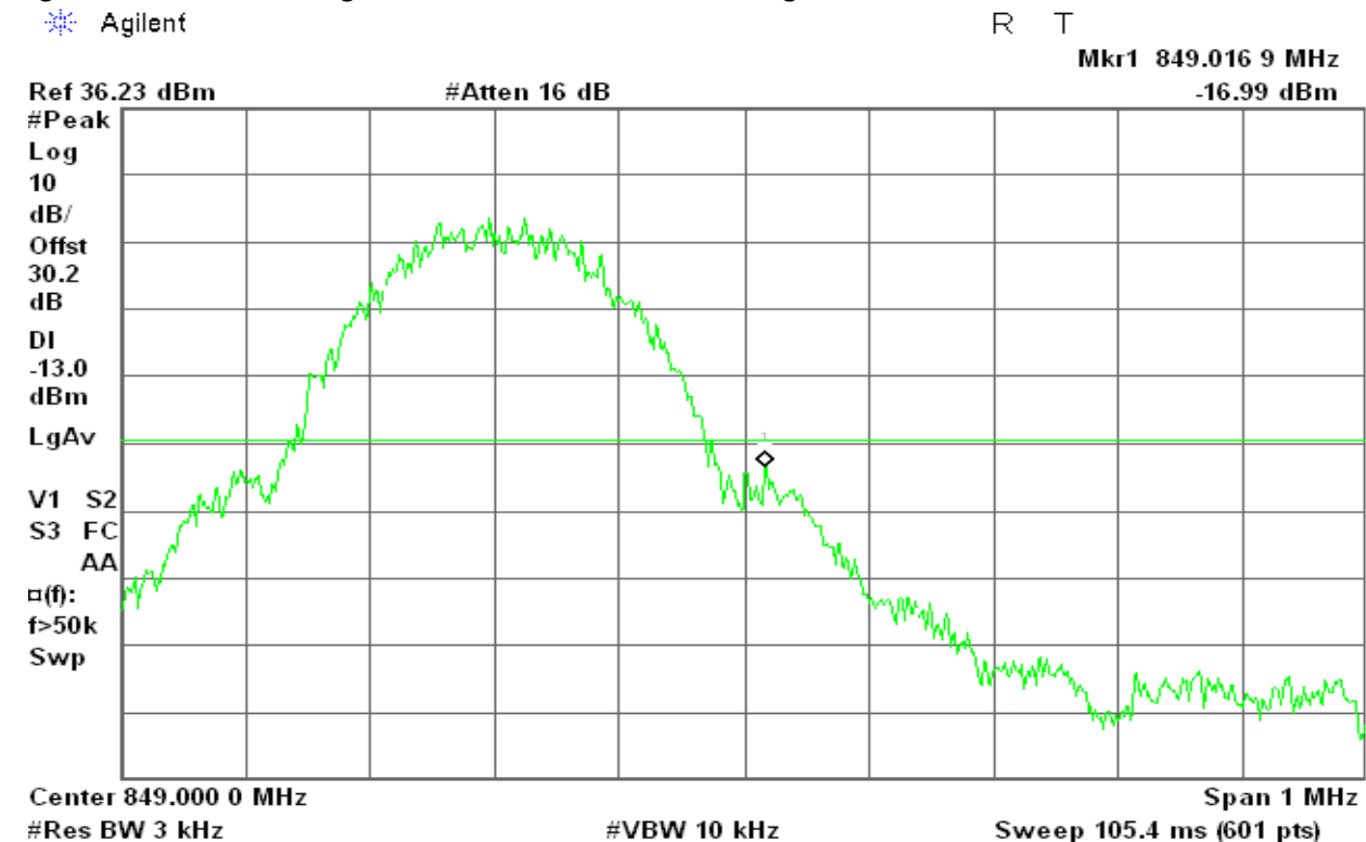
Figure 14-2: Band Edge emissions – EDGE CH High
