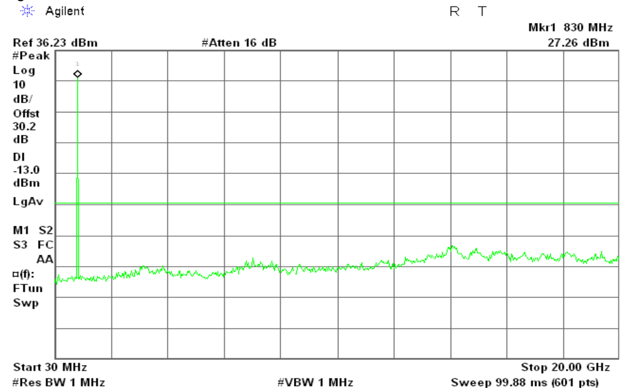
Figure 13-2: Out of Band emission at antenna terminals –EDGE CH Mid
