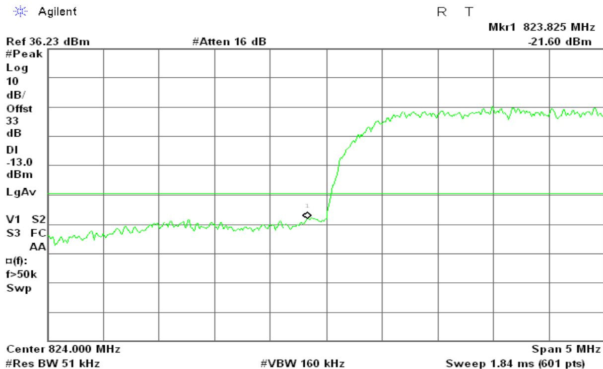
Figure 11-4: Band Edge emissions –WCDMA CH Low
