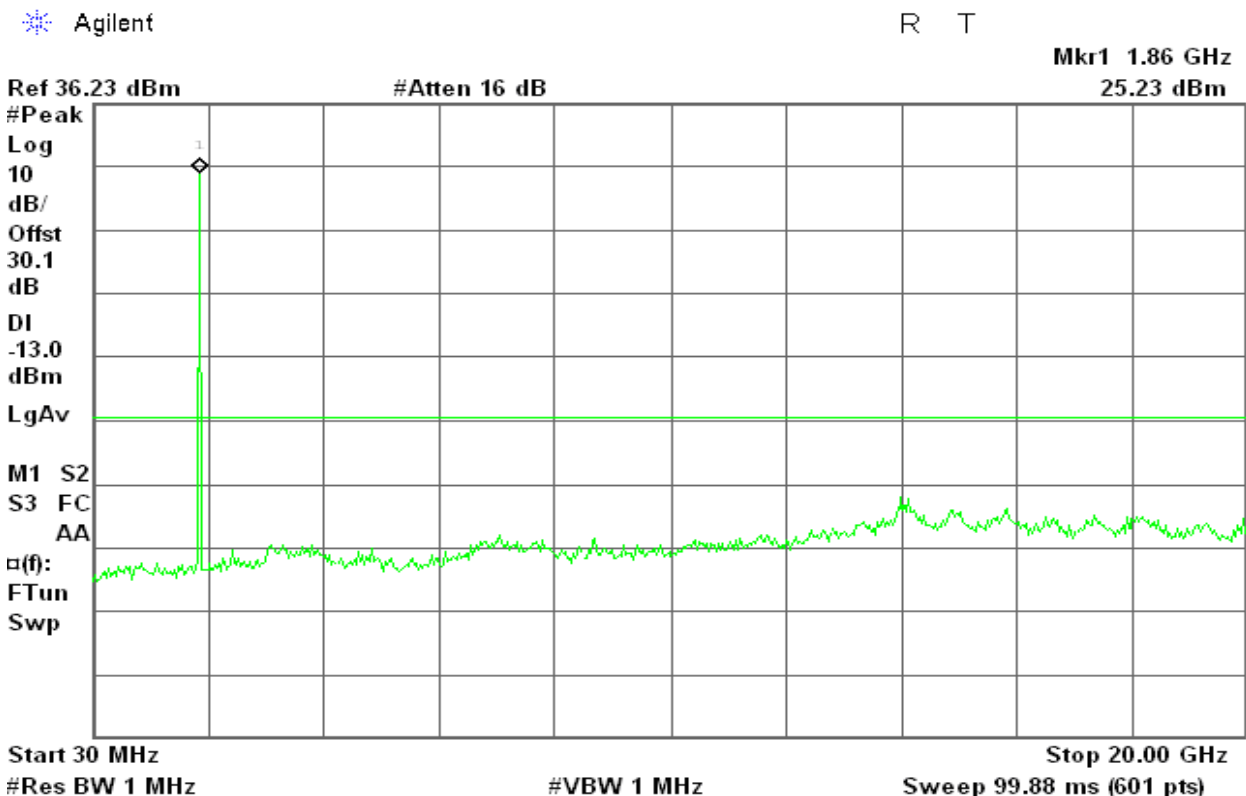
Figure 13-4: Out of Band emission at antenna terminals –EDGE CH Low
