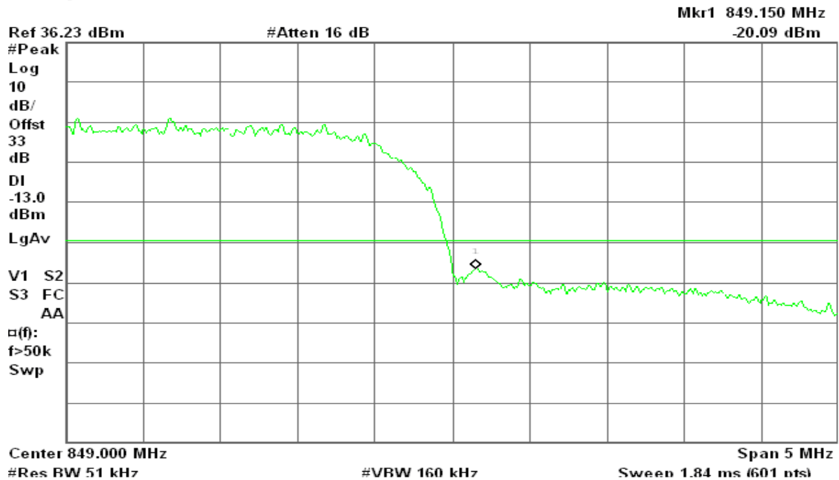
Figure 11-5: Band Edge emissions –WCDMA CH High
