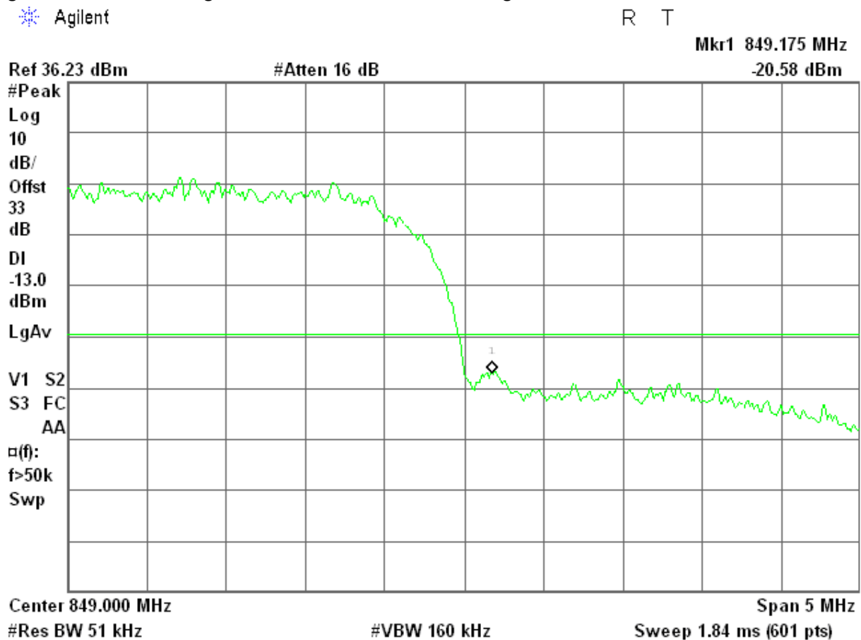
Figure 12-5: Band Edge emissions – HSDPA CH High
