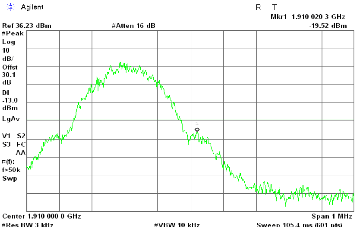
Figure 14-4: Band Edge emissions – EDGE CH High
