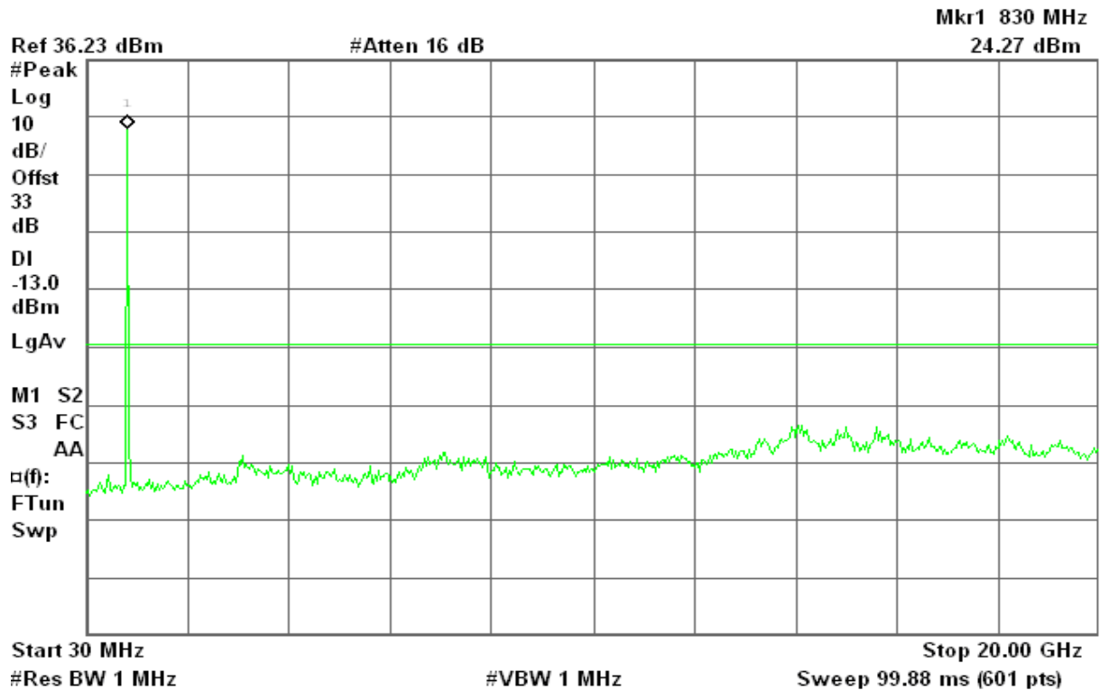
Figure 12-2: Out of Band emission at antenna terminals – HSDPA CH Mid
