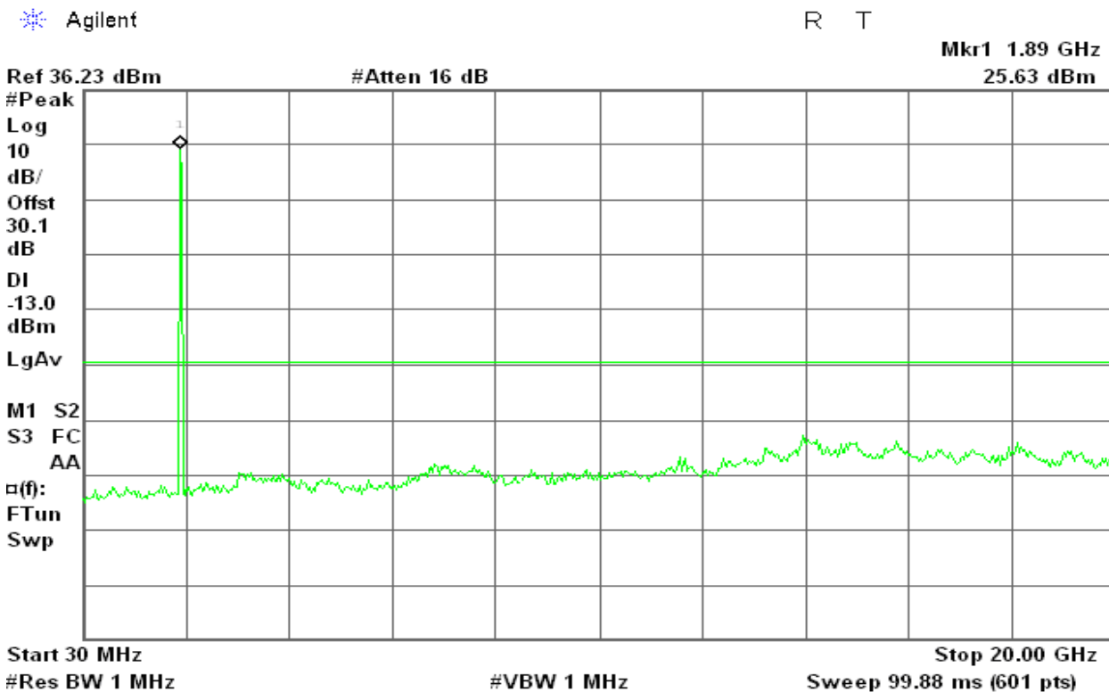
Figure 13-6: Out of Band emission at antenna terminals –EDGE CH High
