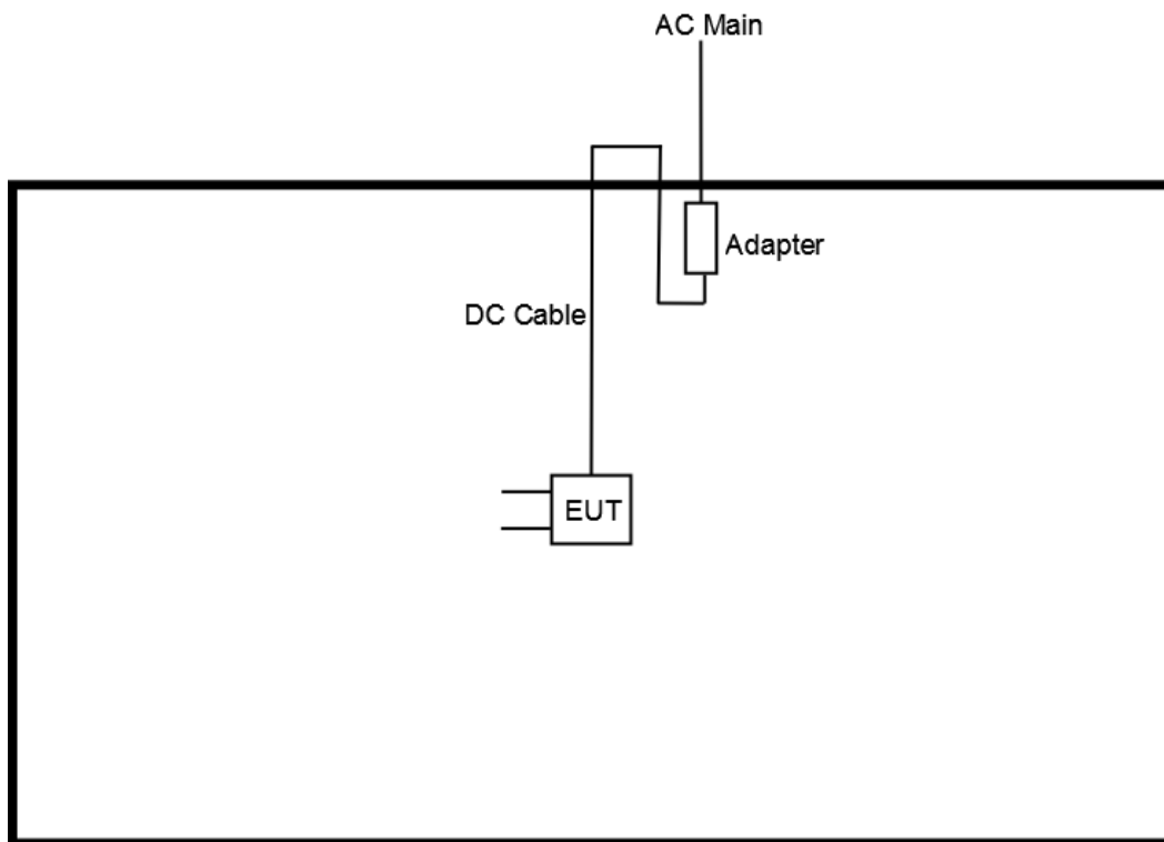
Test Setup Diagram - Radiated Above 1GHz Test (Mode 1)
