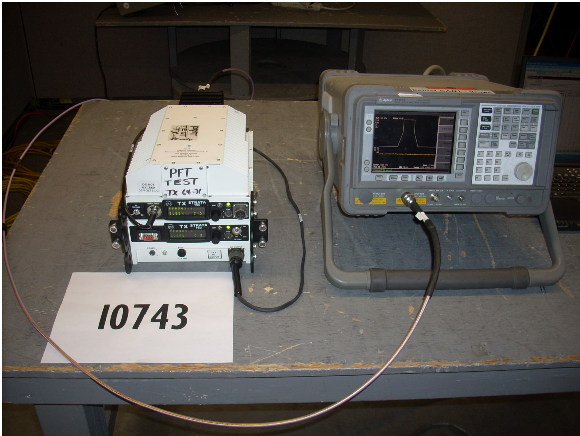
Spectrum Analyzer Measurements – Front
