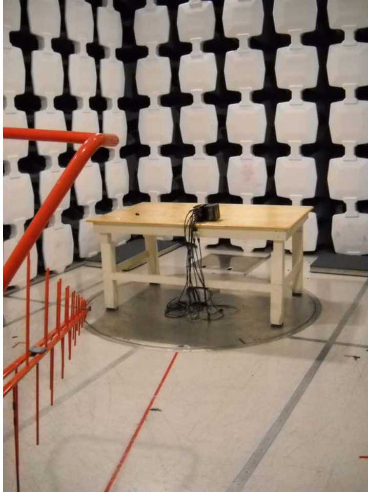
Radiated Emissions - Rear
