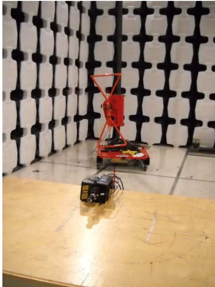
Radiated Emissions - Front
