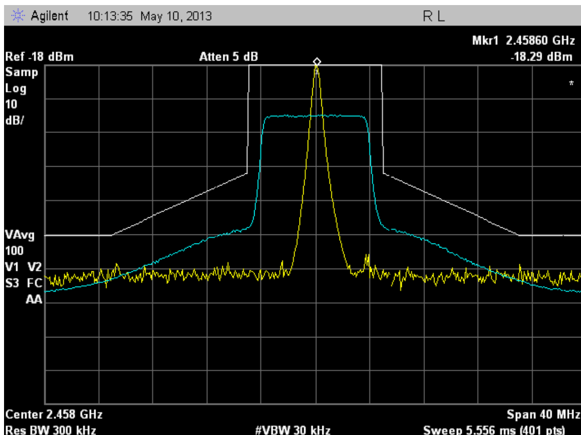
HDX1100 (S Band Channel 8) 10MHz Emission Plot: RF Power = 36.6dBm / 4.5W
