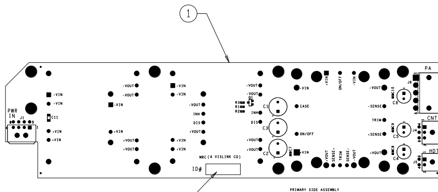
PRIMARY SIDE ASSEMBLY
