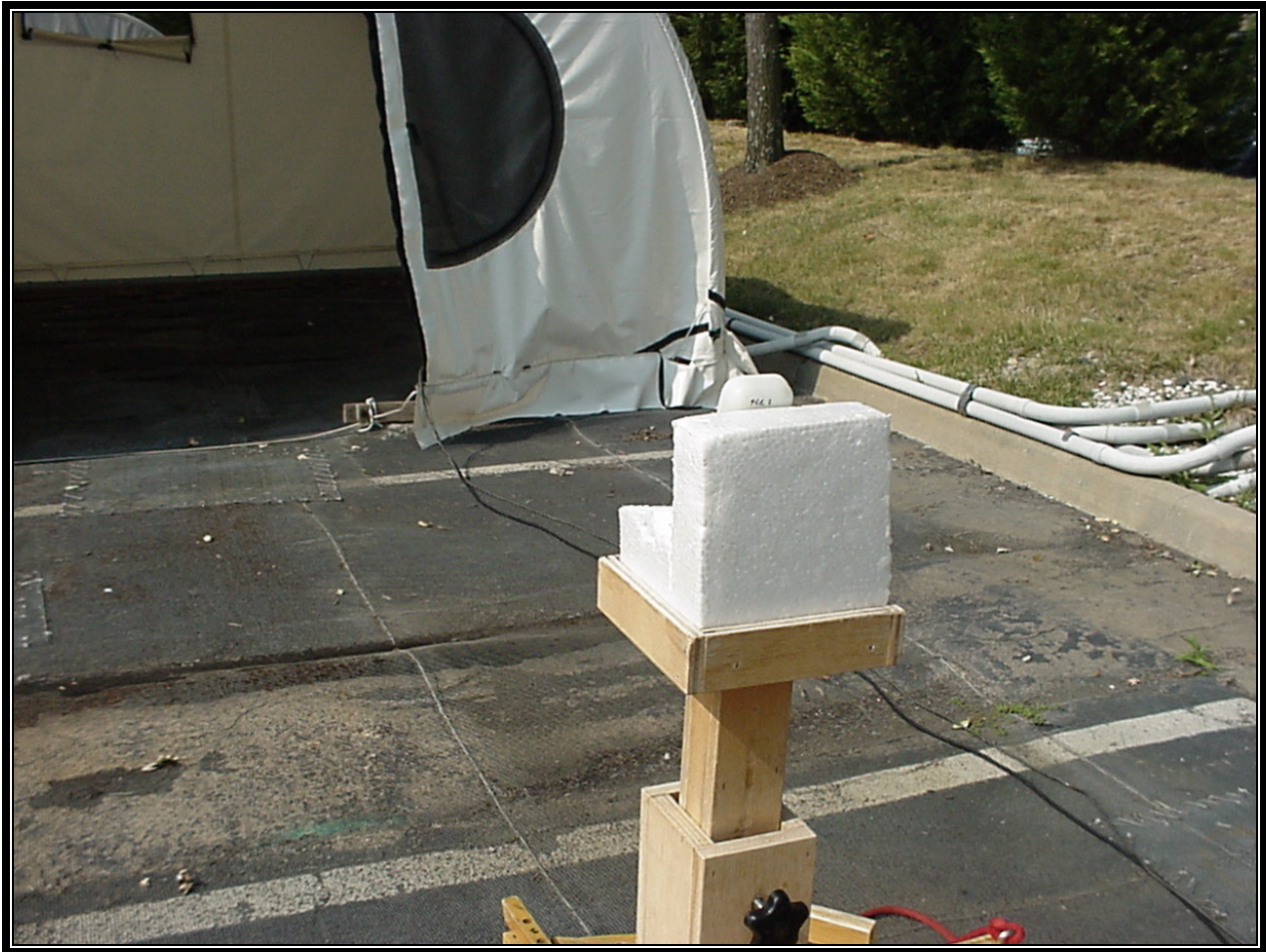
Photograph 3: Radiated Testing – Back View
