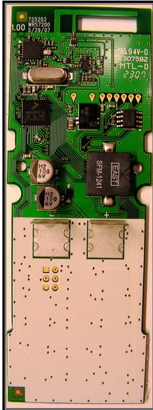
Photograph 11: Keypad PCB Back
