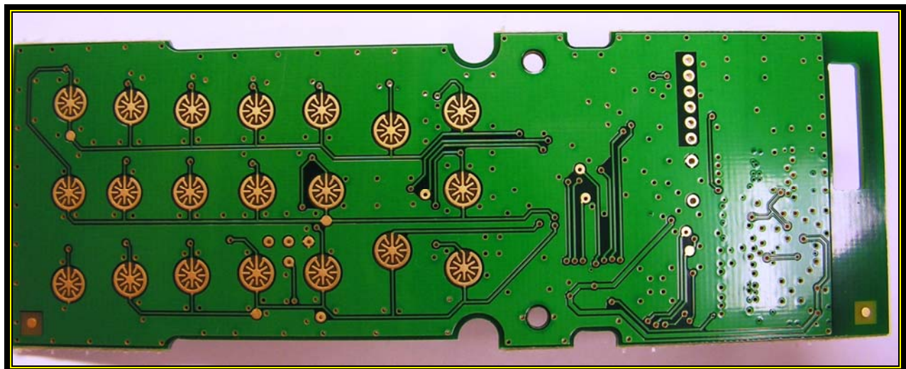
Photograph 13: Keypad PCB Front without LCD
