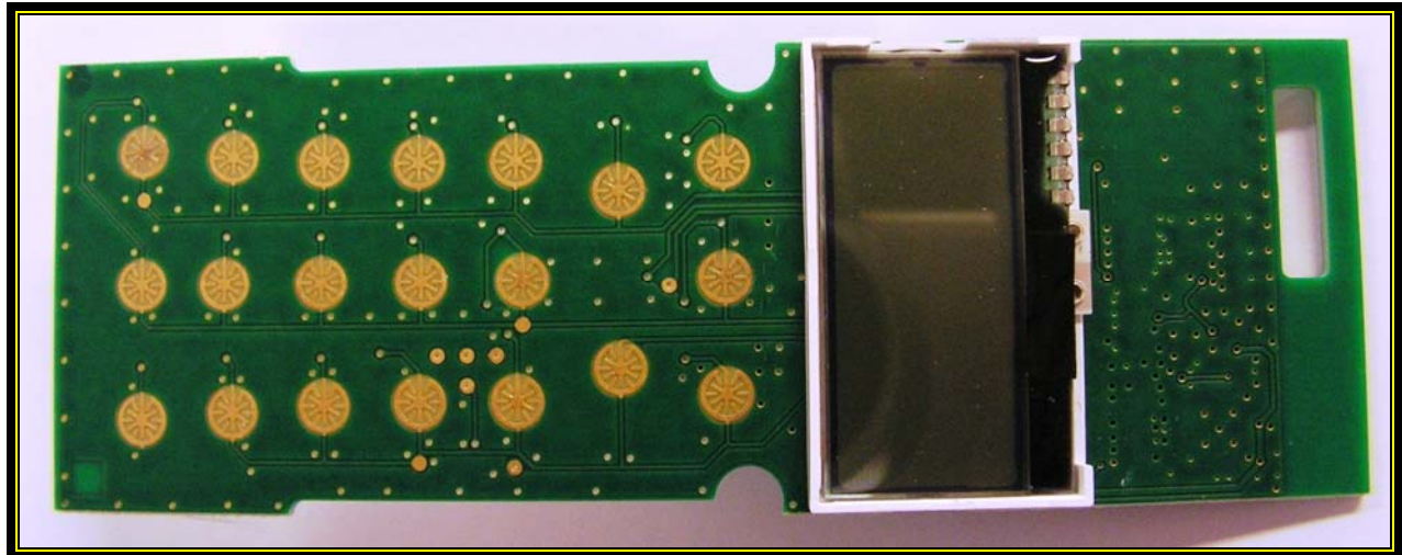
Photograph 12: Keypad PCB Front with LCD
