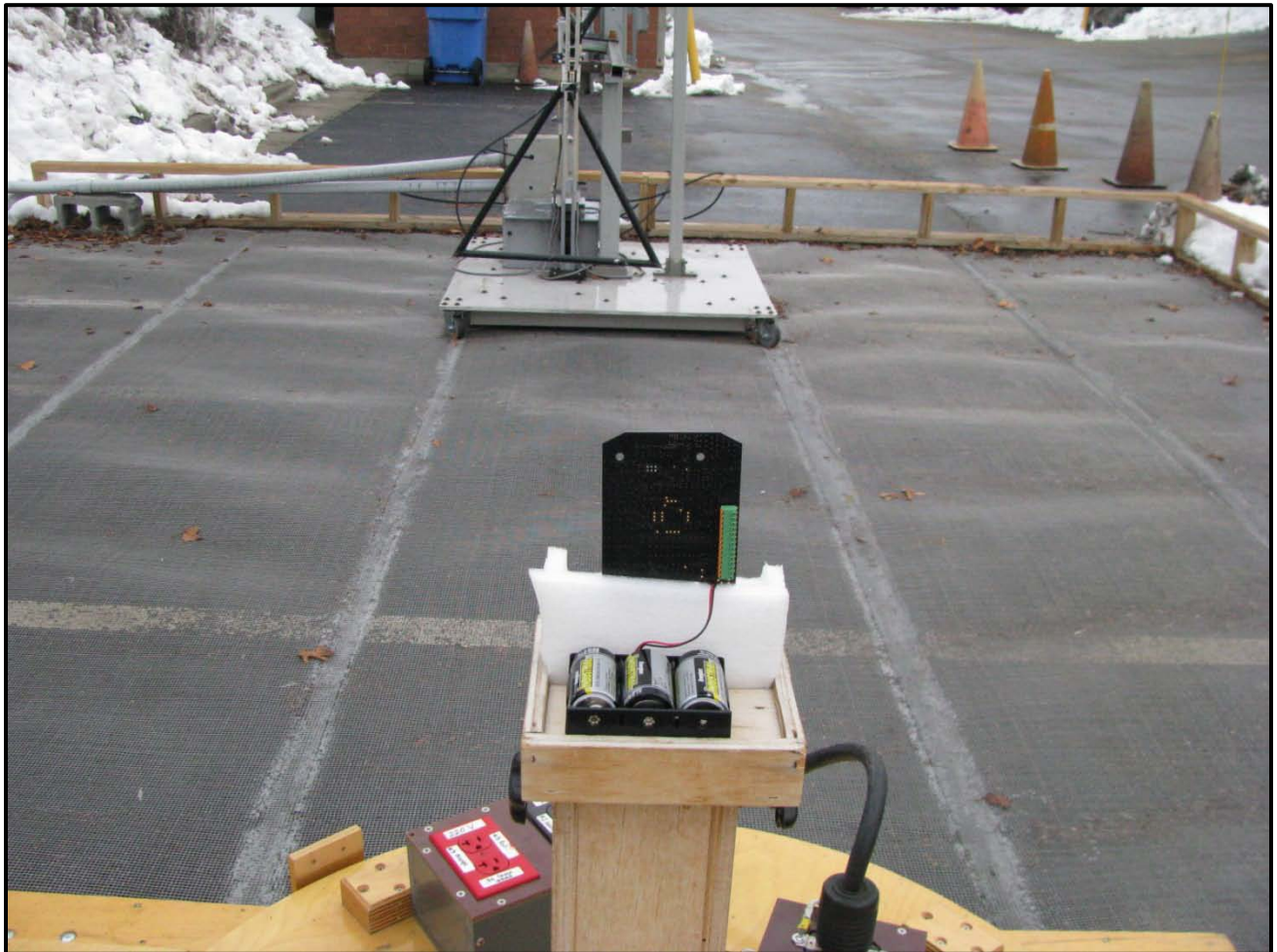
Photograph 3: Radiated Testing – Back View
