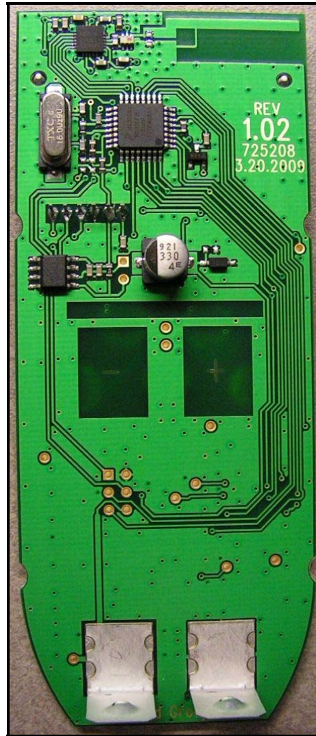
Photograph 11: Transmitter Module – Bottom View
