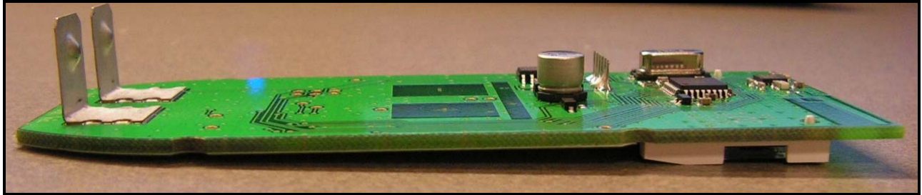
Photograph 12: Transmitter Module - Side View
