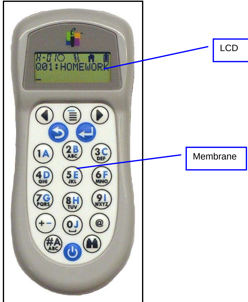
Photograph 8: Top of Case of "Typical Host"
