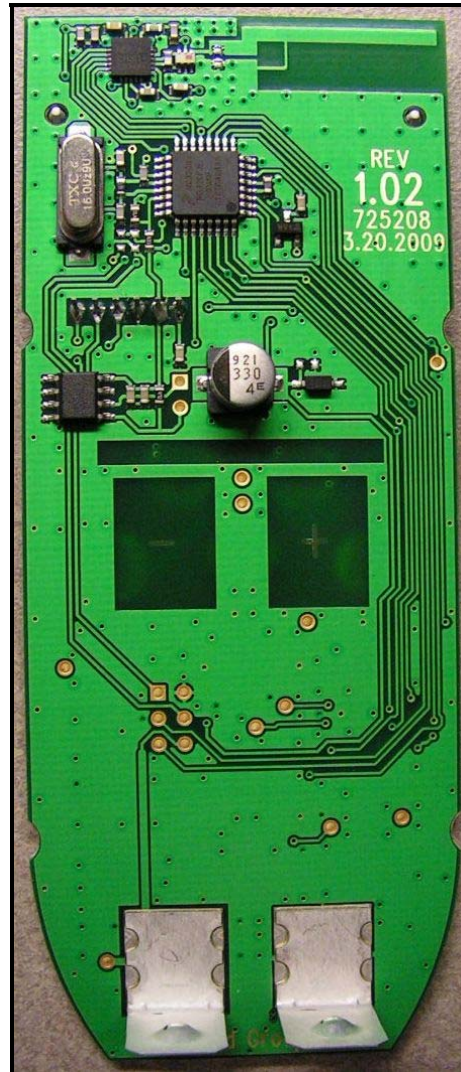
Photograph 6: Transmitter Module – Bottom View
