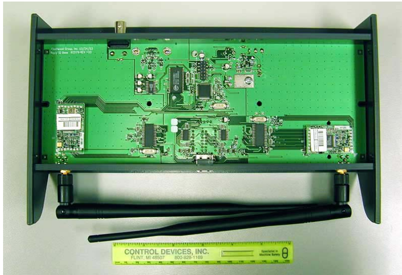
Base Circuit Board Component Side
